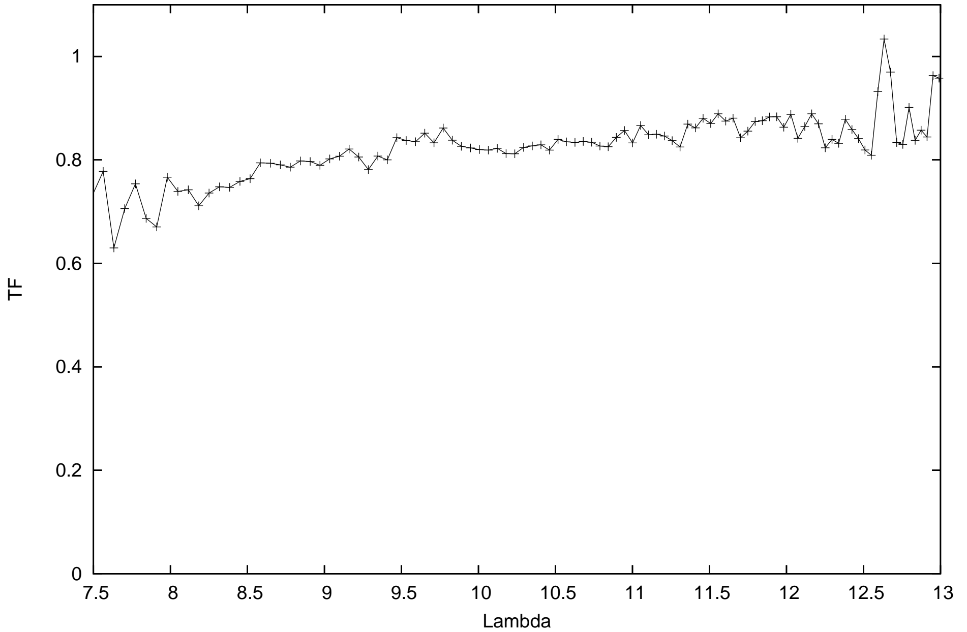
calHD029139_flux-3.11_diam20.4_r.MIDI.2011-01-28T01_11_48.137_A1B2
