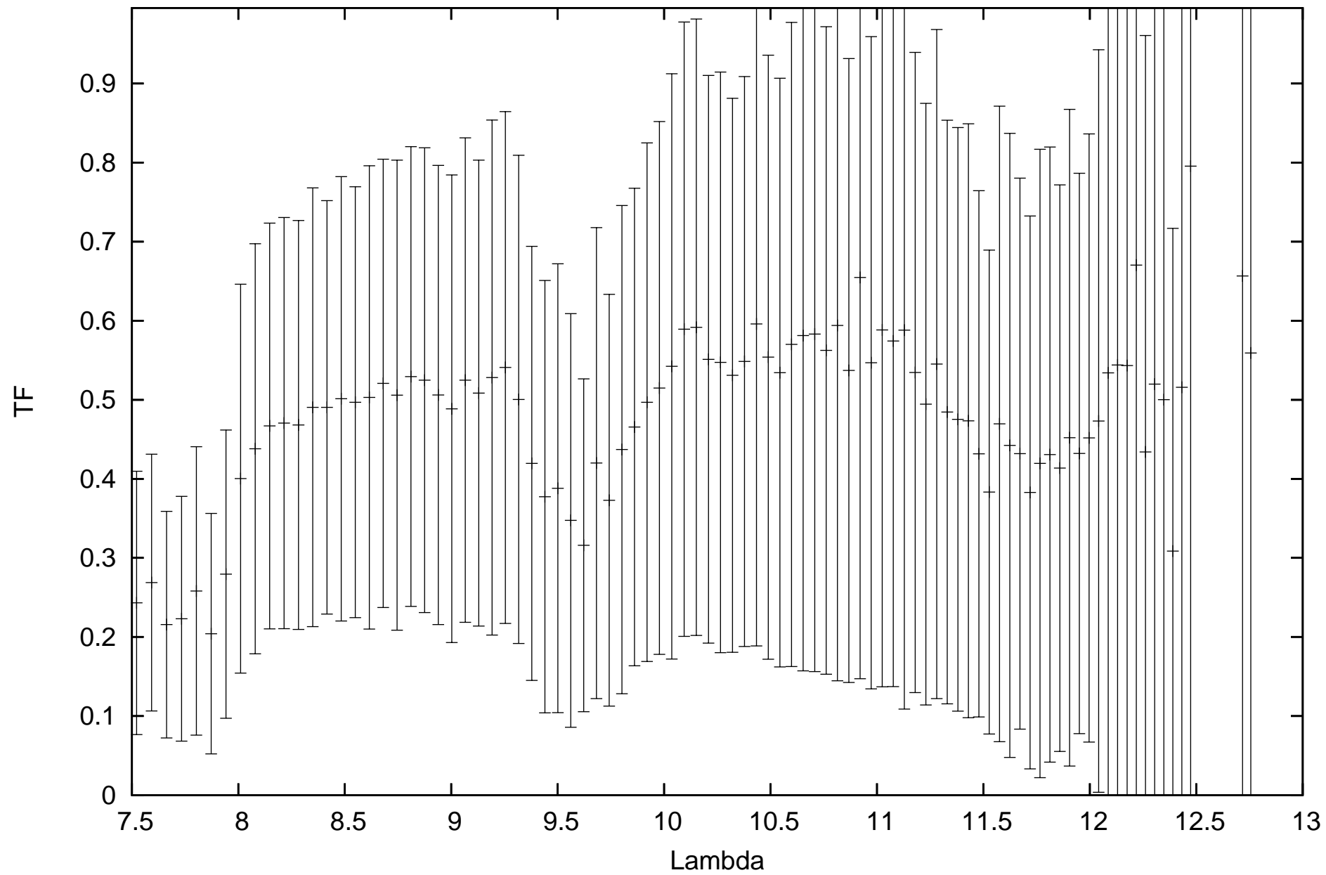
calHD125687_flux0.4_diam4.03_r.MIDI.2011-05-06T03_41_45.000_D0B2
