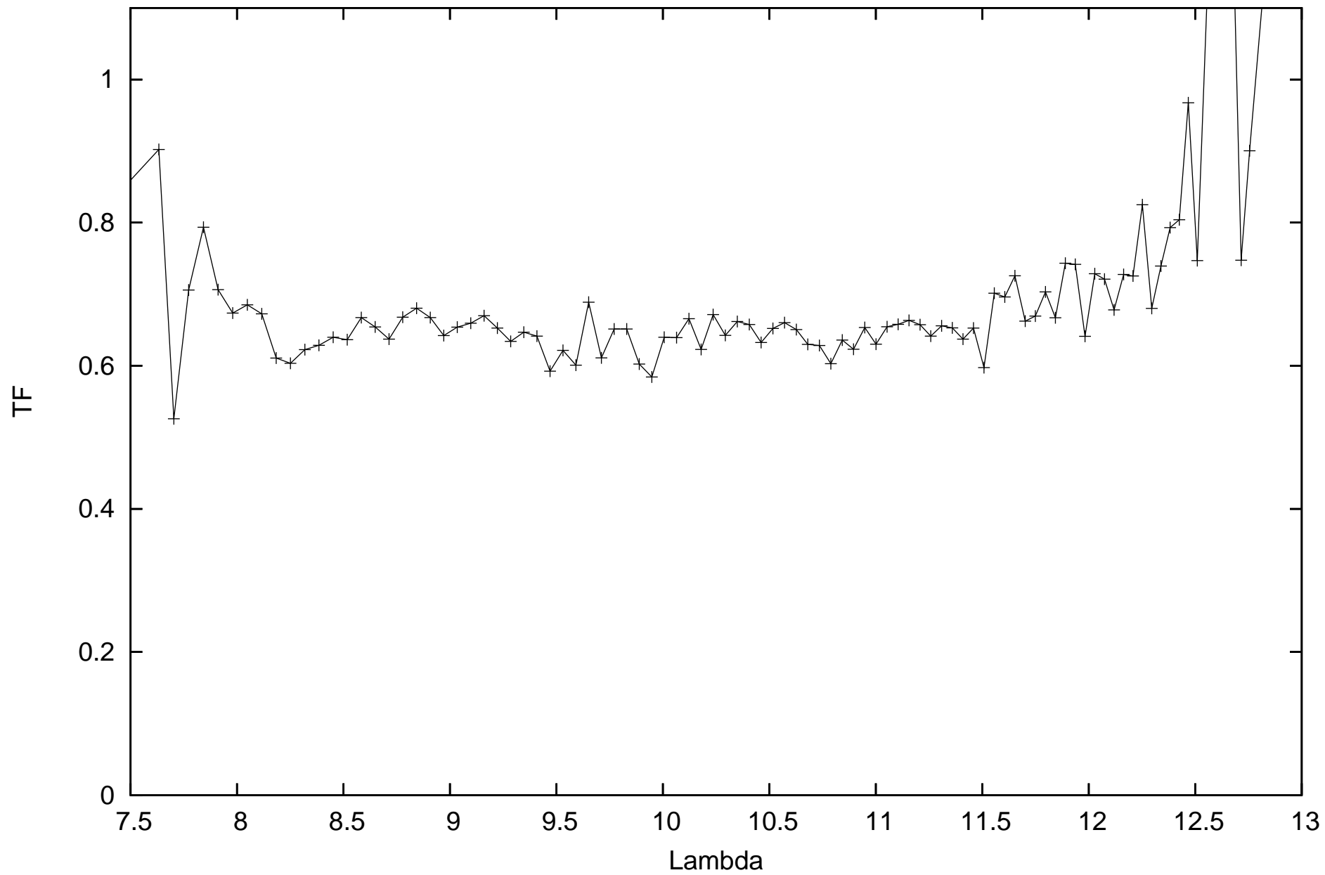
calHD167618_flux-1.82_diam11.66_r.MIDI.2011-05-31T09_42_27.138_D0G1
