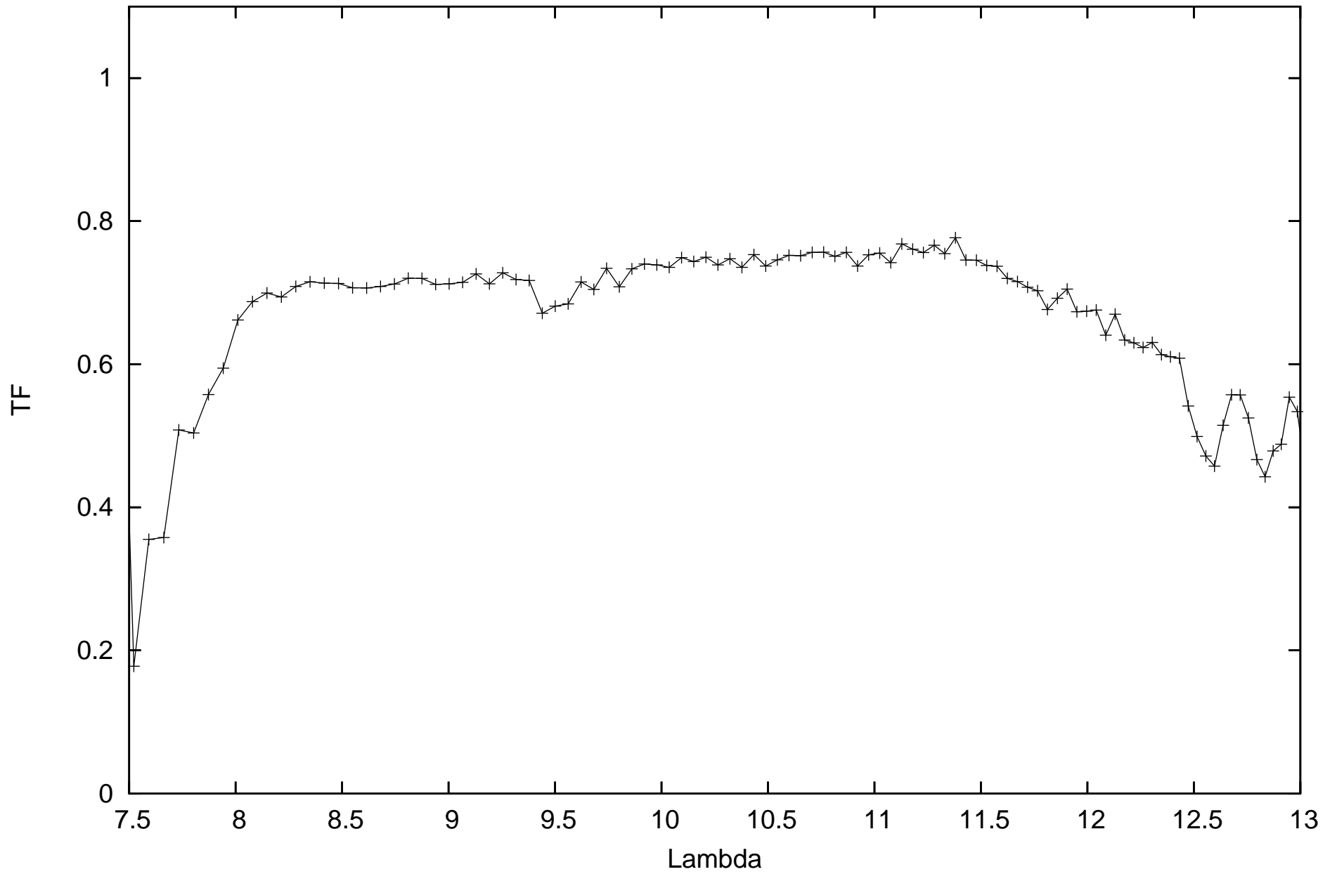
calHIP82363_flux-0.3207_diam5.52_r.MIDI.2011-05-31T08_10_42.000_H0G1
