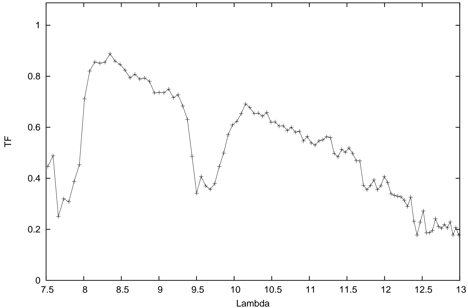
calHIP82363_flux-0.3207_diam5.52_r.MIDI.2011-05-31T09_14_32.000_DOG1
