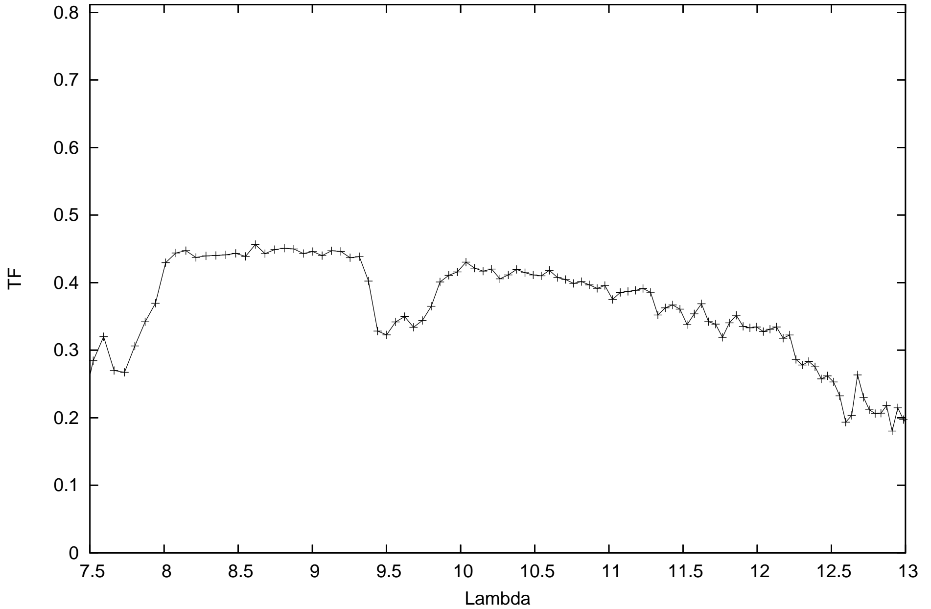
calHIP74745_flux3.11742_diam1.148885_r.MIDI.2011-06-15T04_30_20.000_U1U4
