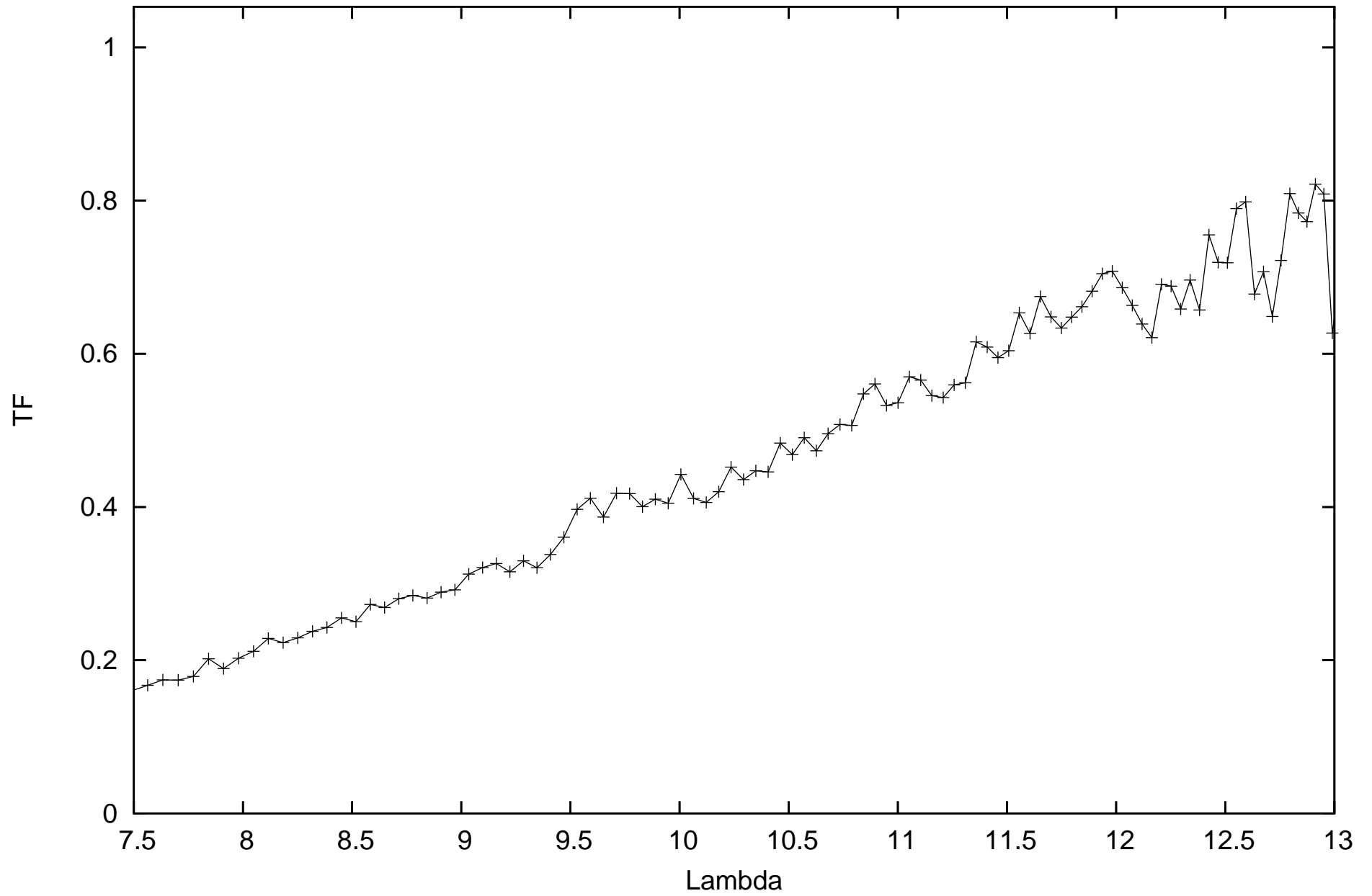
calHD167618_flux-1.82_diam11.66_r.MIDI.2011-06-24T08_58_40.138_G111
