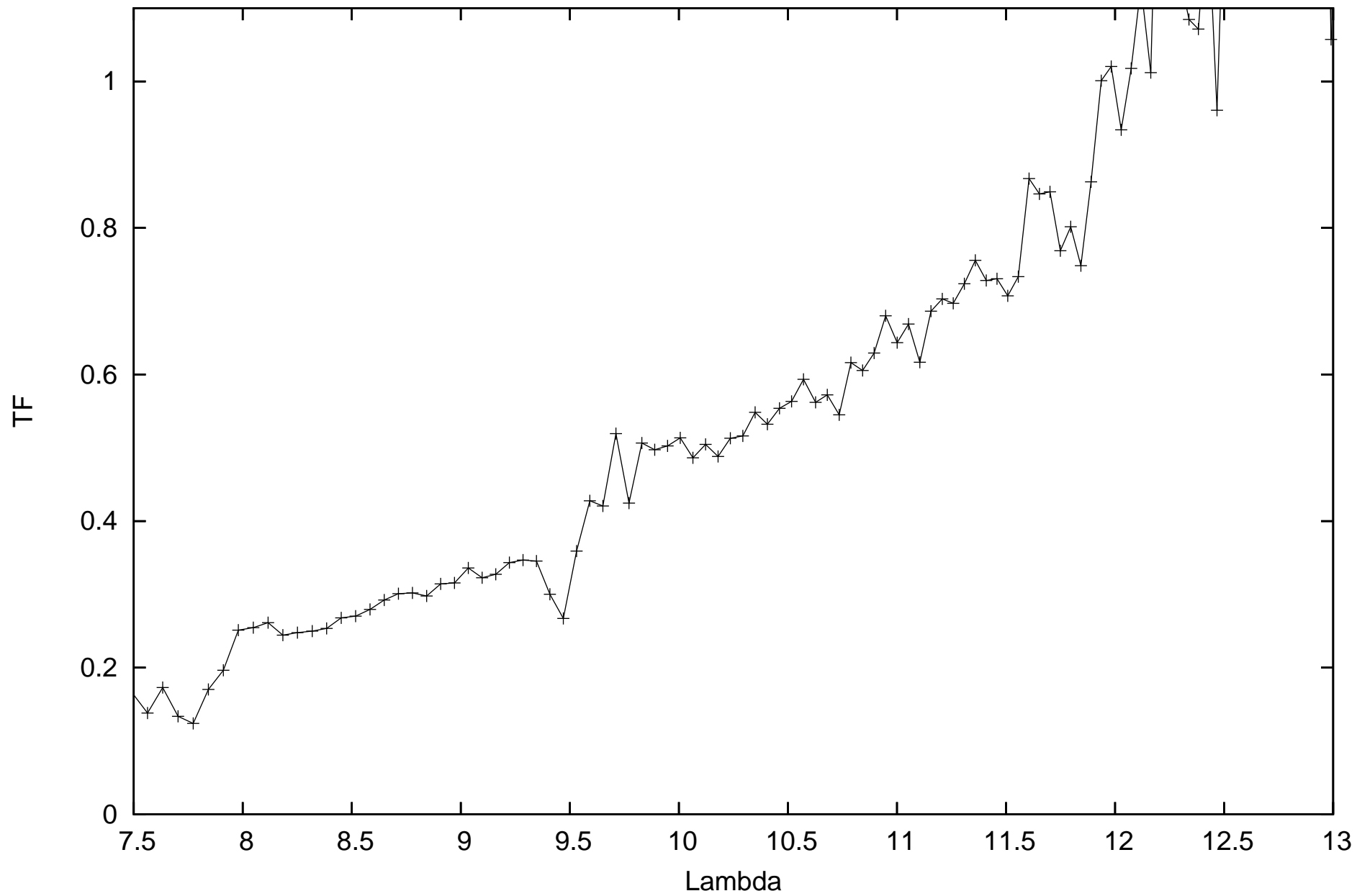
calHD167618_flux-1.82_diam11.66_r.MIDI.2011-06-24T09_26_38.137_G1A1
