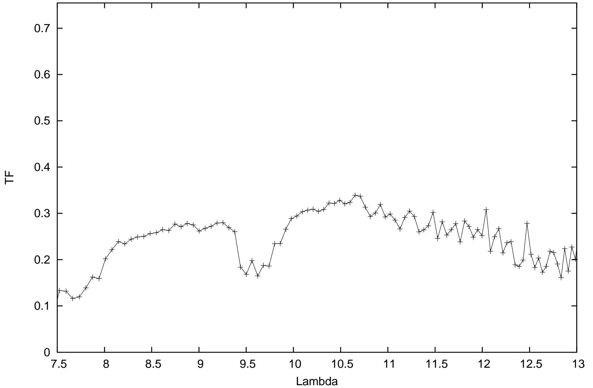
calHIP82363_flux-0.3207_diam5.52_r.MIDI.2011-07-02T04_05_40.000_DOG1
