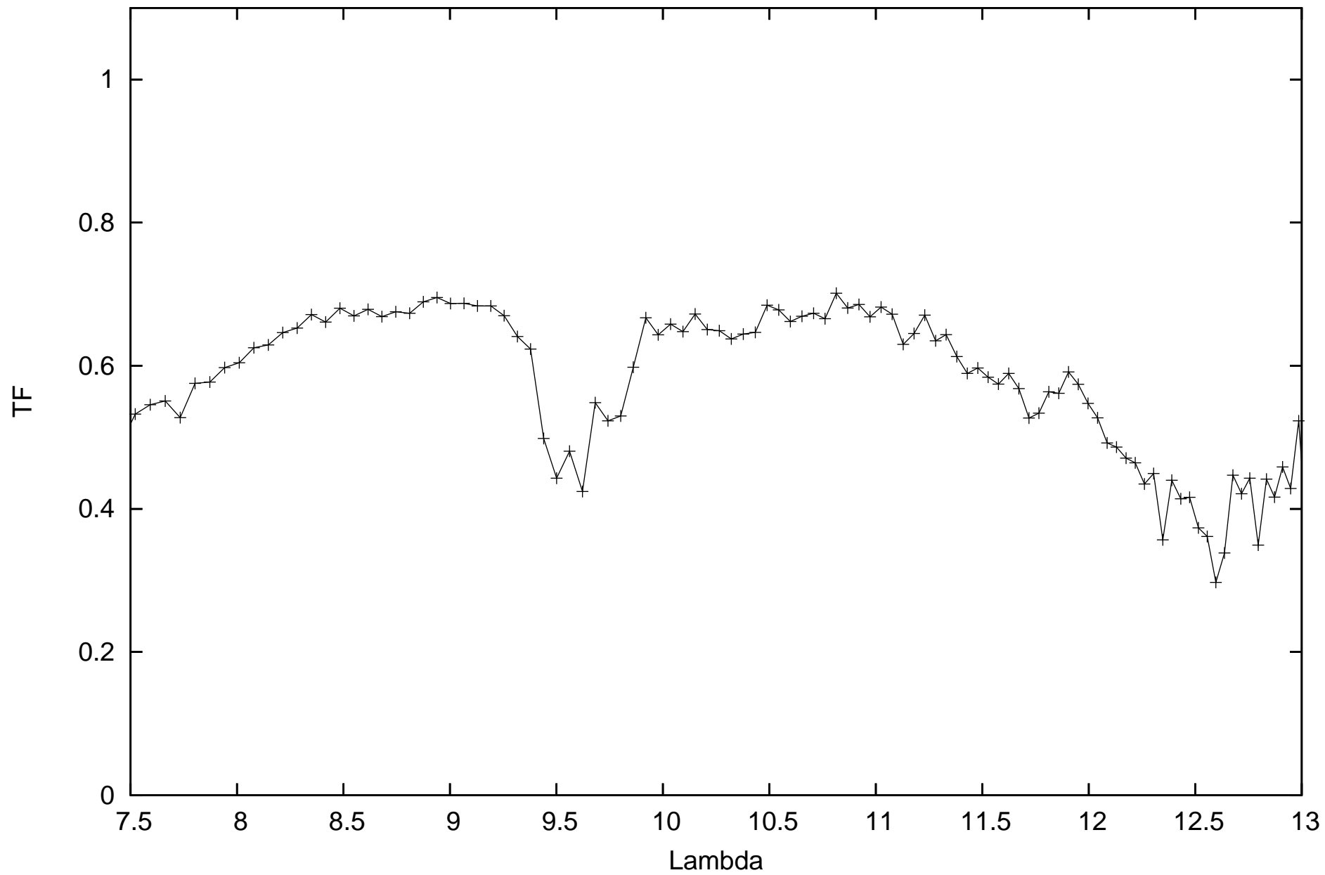
calHIP90496_flux0.238088_diam3.99_r.MIDI.2011-07-26T06_04_12.000_K0I1
