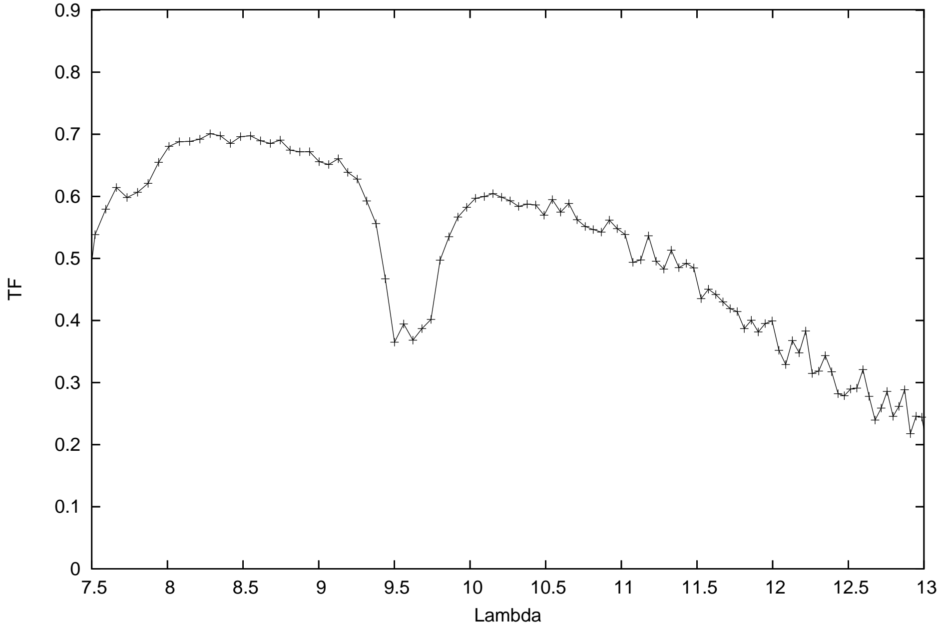
calHIP90496_flux0.238088_diam3.99_r.MIDI.2011-07-26T06_49_19.000_G111
