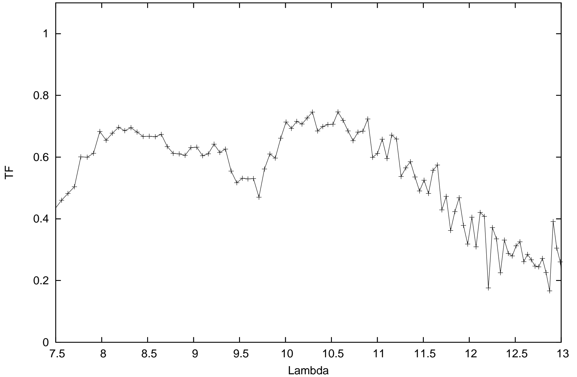
calHD224935_flux-0.85_diam7.24_r.MIDI.2011-08-13T08_58_51.179_C1B2
