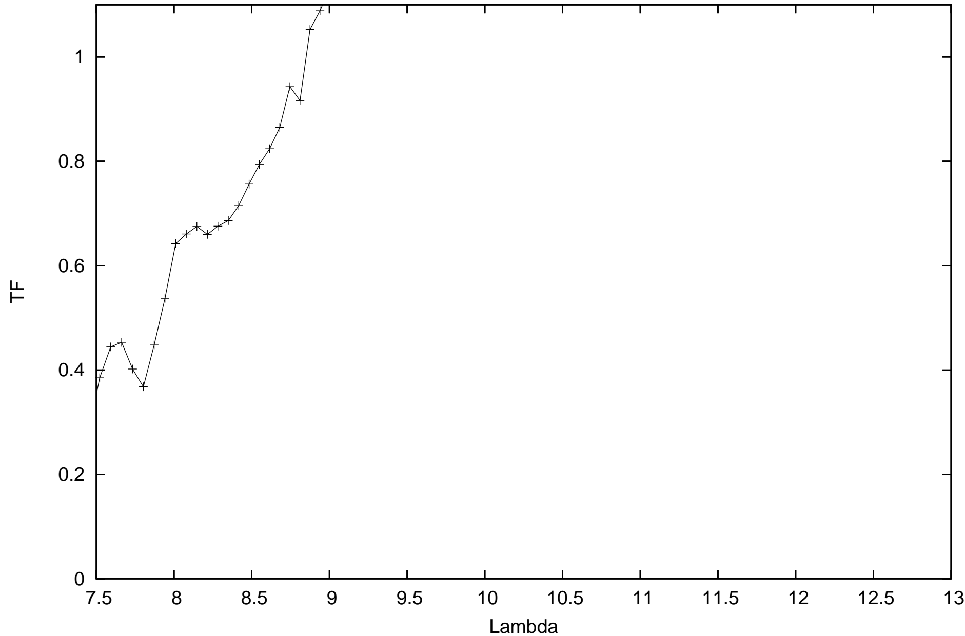
calHIP97278_flux-0.73709_diam7.256253_r.MIDI.2011-09-01T02_53_28.000_I1A1
