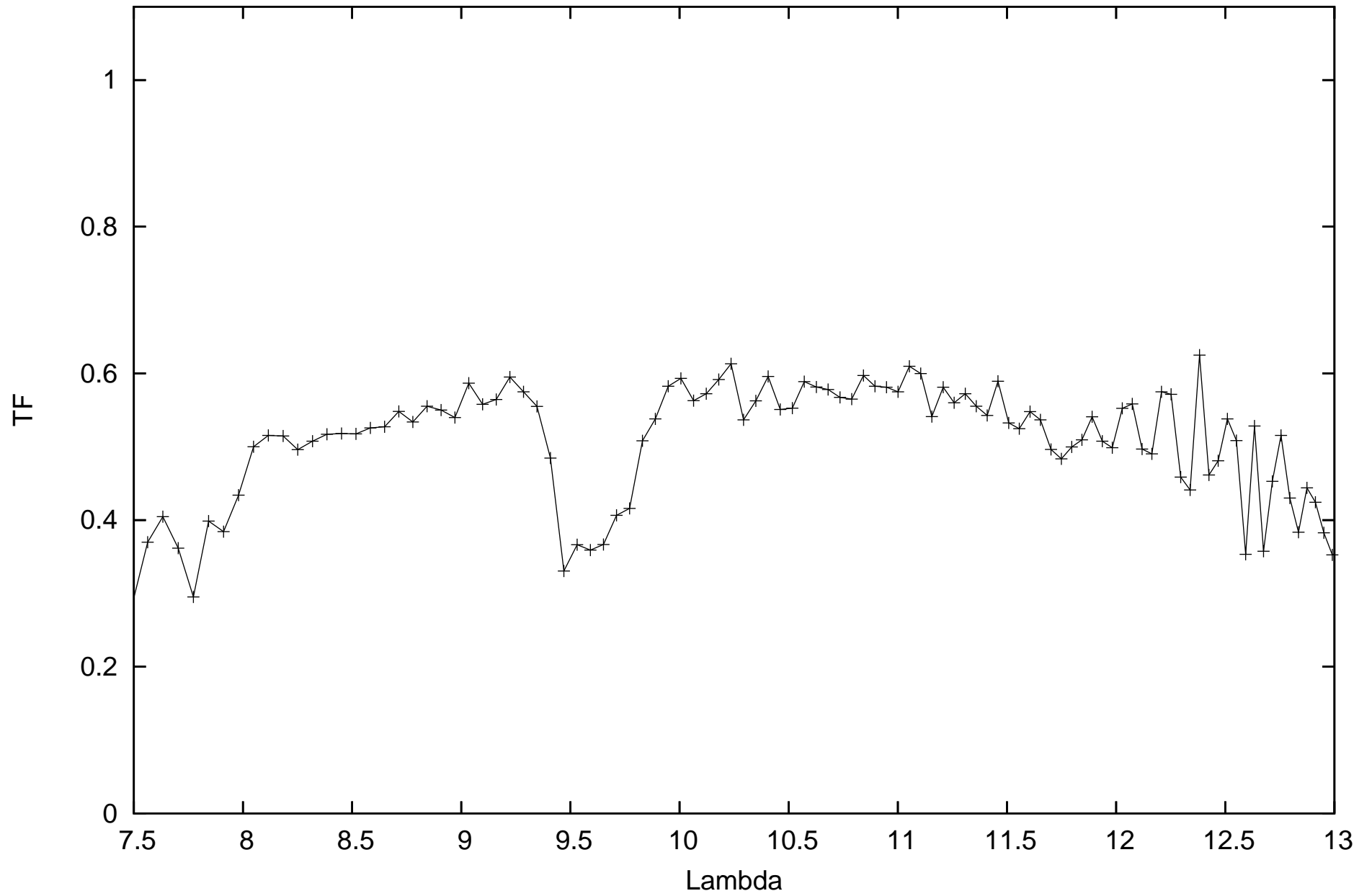
calHIP89931_flux-0.511_diam5.87_r.MIDI.2011-10-20T01_50_09.135_K011
