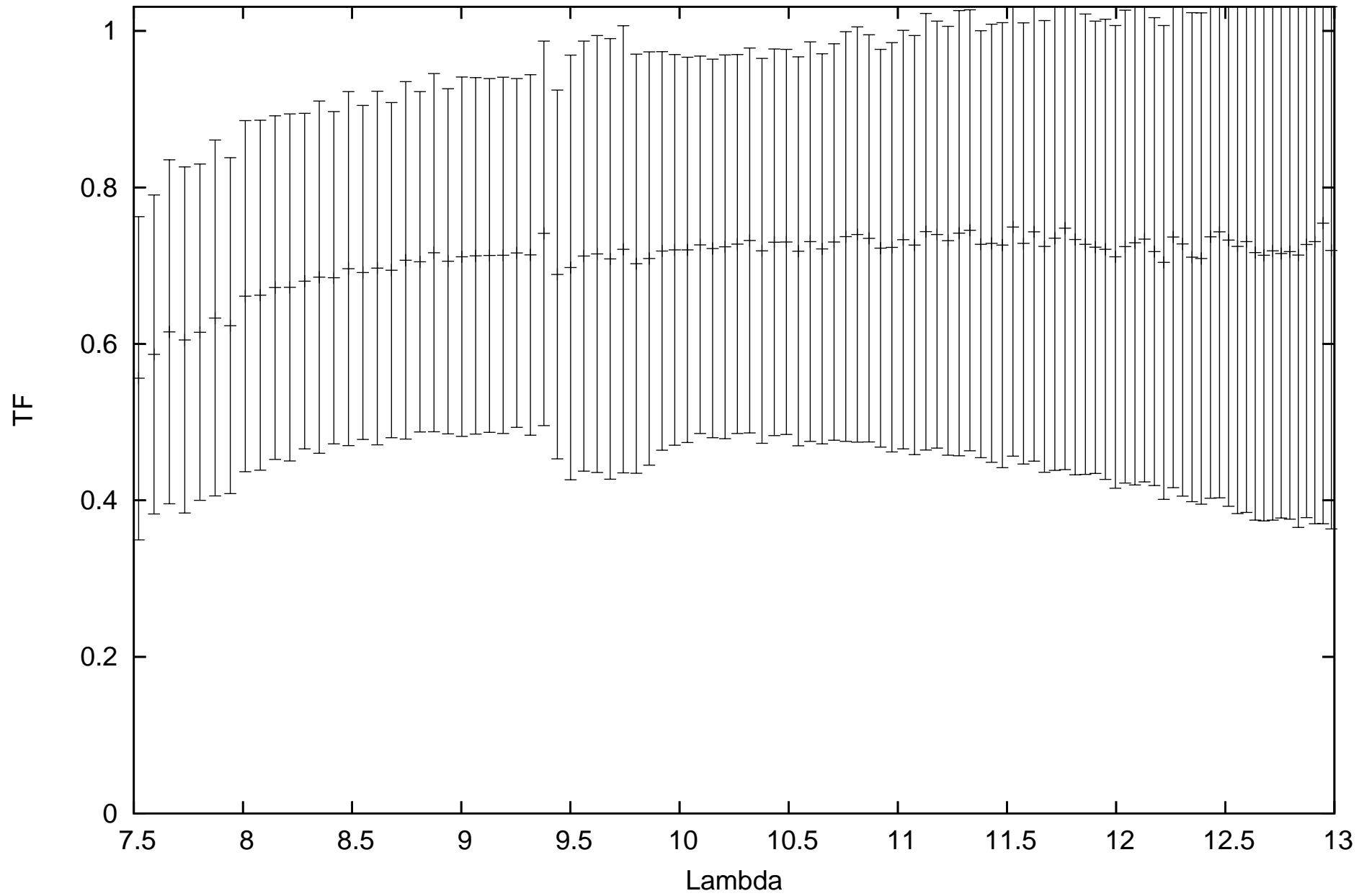
calHD167618_flux-1.82_diam11.66_r.MIDI.2011-10-22T23_54_44.000_C1A1
