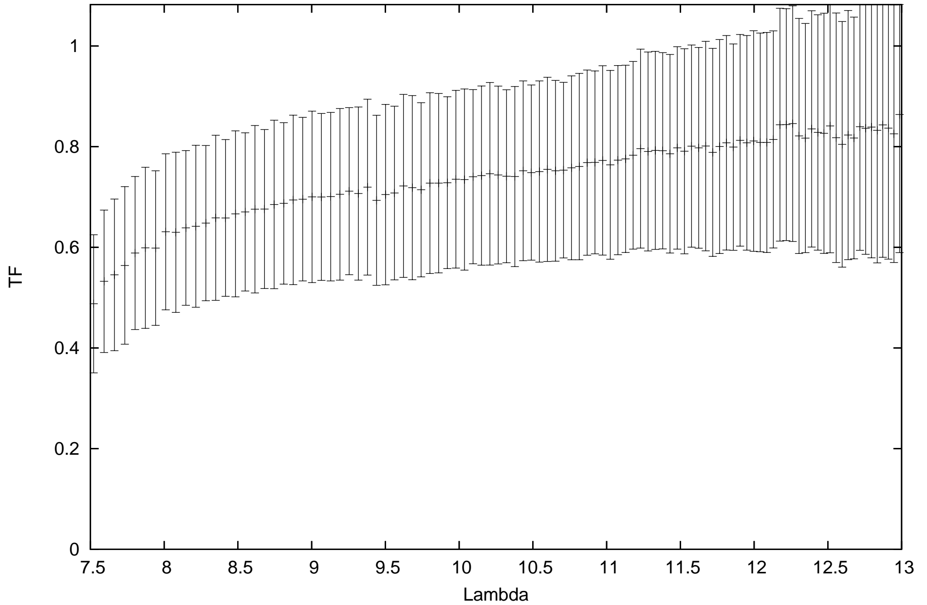
calHD018884_flux-1.93_diam12.27_r.MIDI.2011-01-05T01_40_14.000_I1E0
