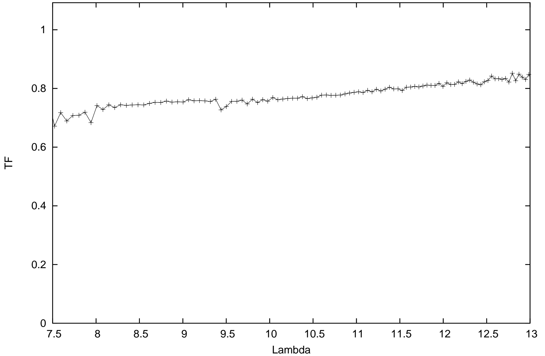
calHD029139_flux-3.11_diam20.4_r.MIDI.2011-01-28T01_03_08.000_A1B2
