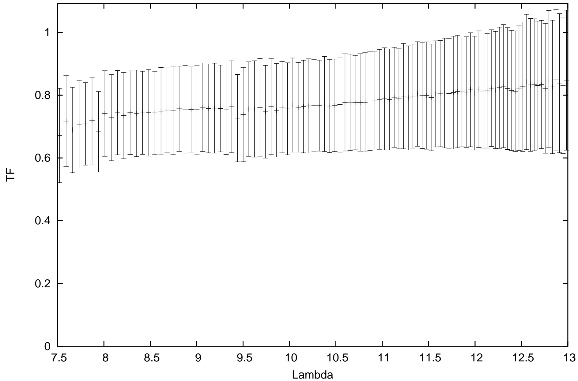
calHD029139_flux-3.11_diam20.4_r.MIDI.2011-01-28T01_03_08.000_A1B2
