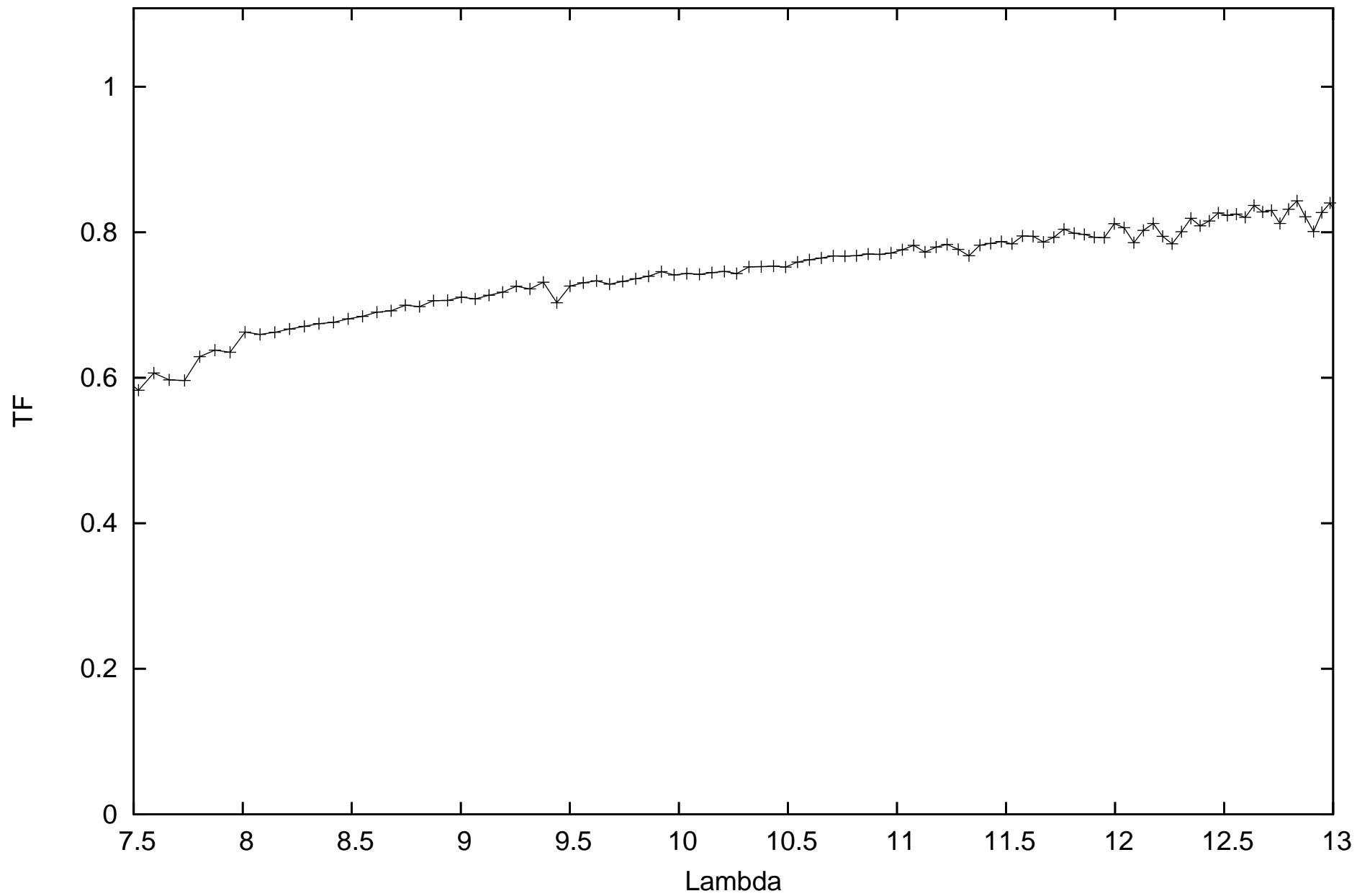
calHD044478_flux-2.21_diam13.94_r.MIDI.2011-01-05T04_50_15.000_H0G0
