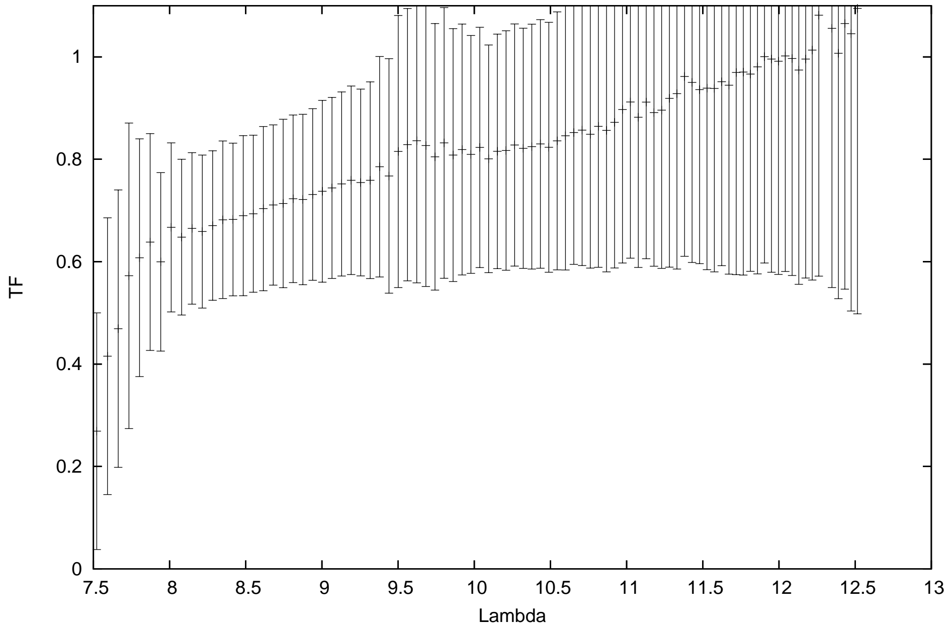
calHD045348_flux-1.47_diam6.87_r.MIDI.2011-02-06T03_38_50.000_A011
