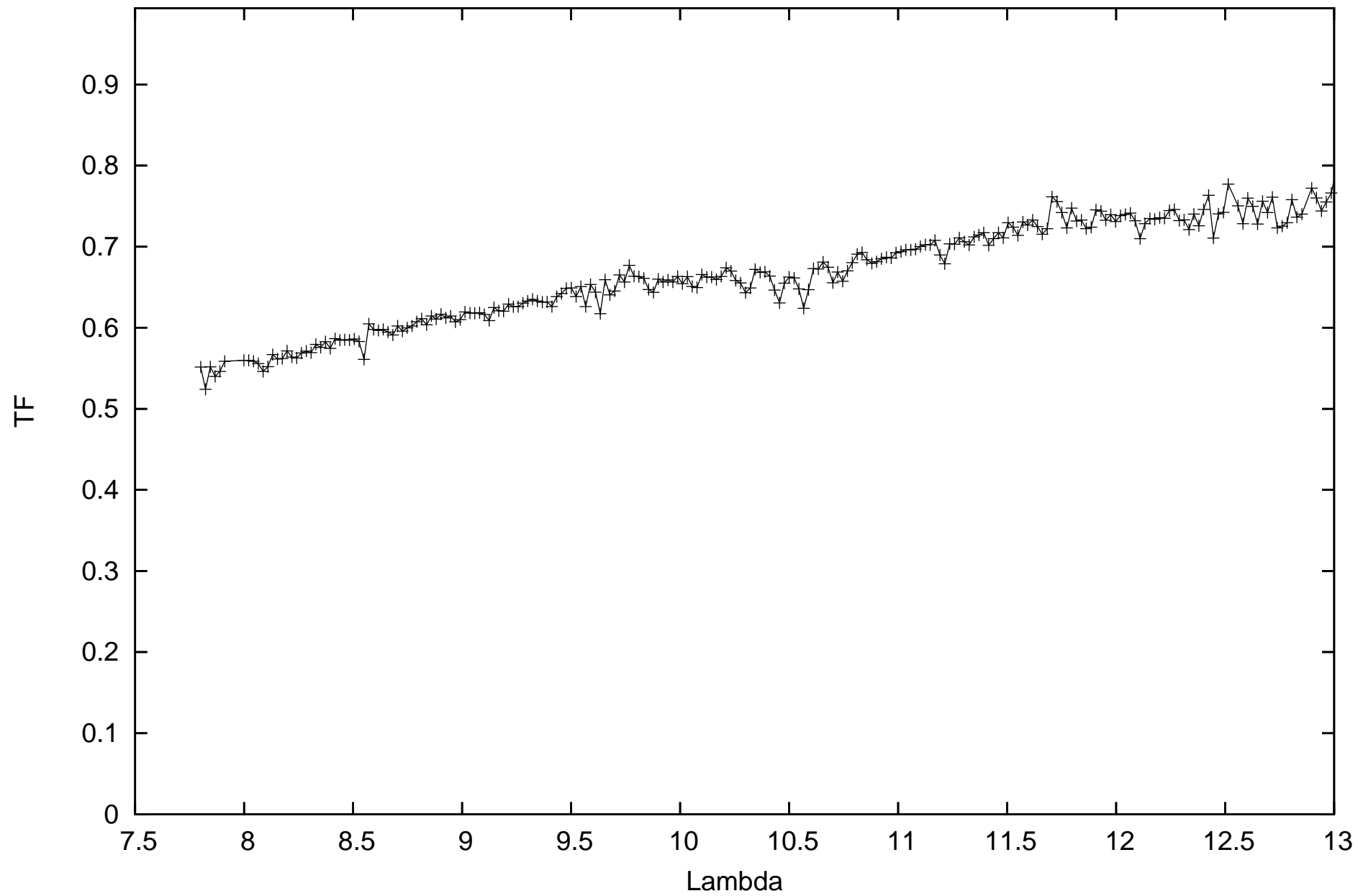
calHDO46612_flux1.15_diam3.12_r.MIDI.2011-01-15T05_08_35.000_U2U3
