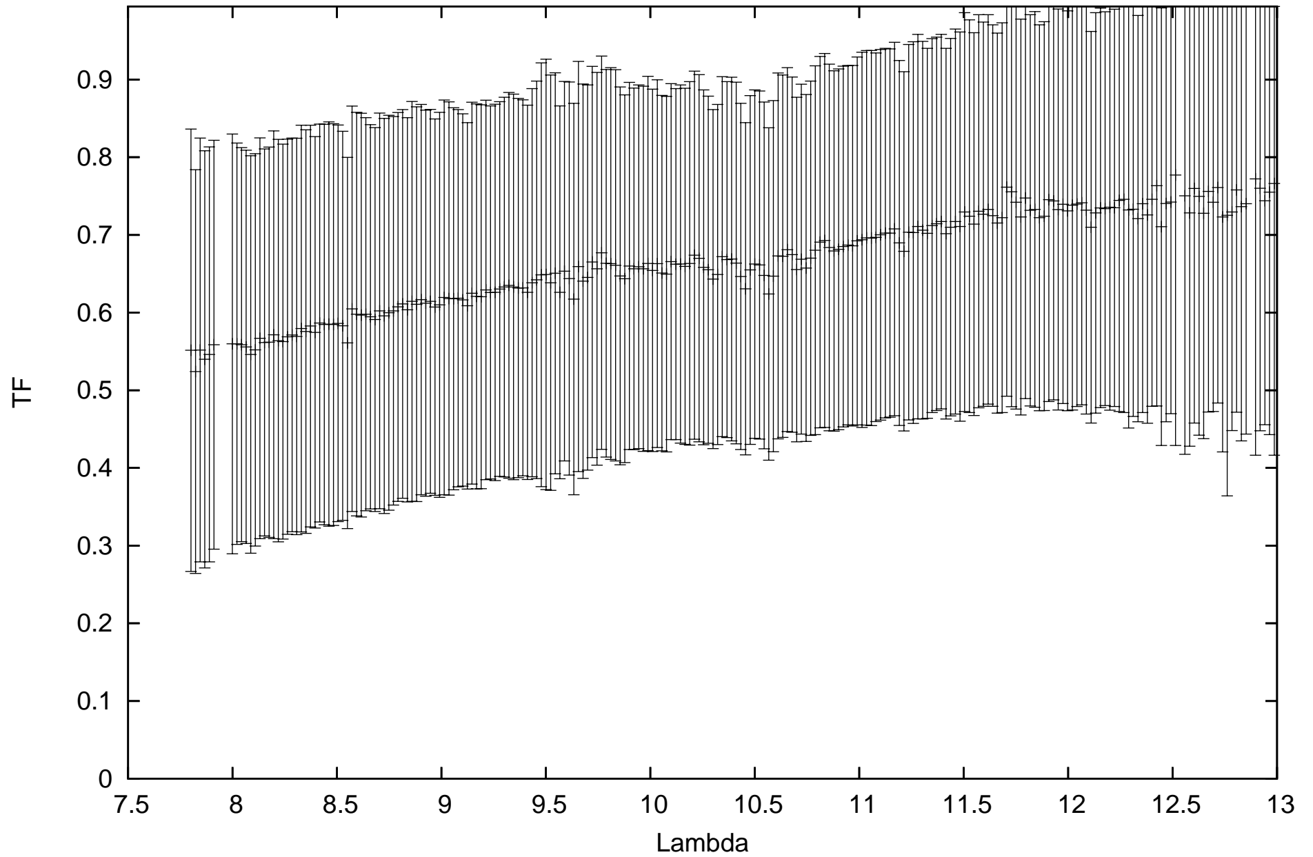
calHD046612_flux1.15_diam3.12_r.MIDI.2011-01-15T05_08_35.000_U2U3
