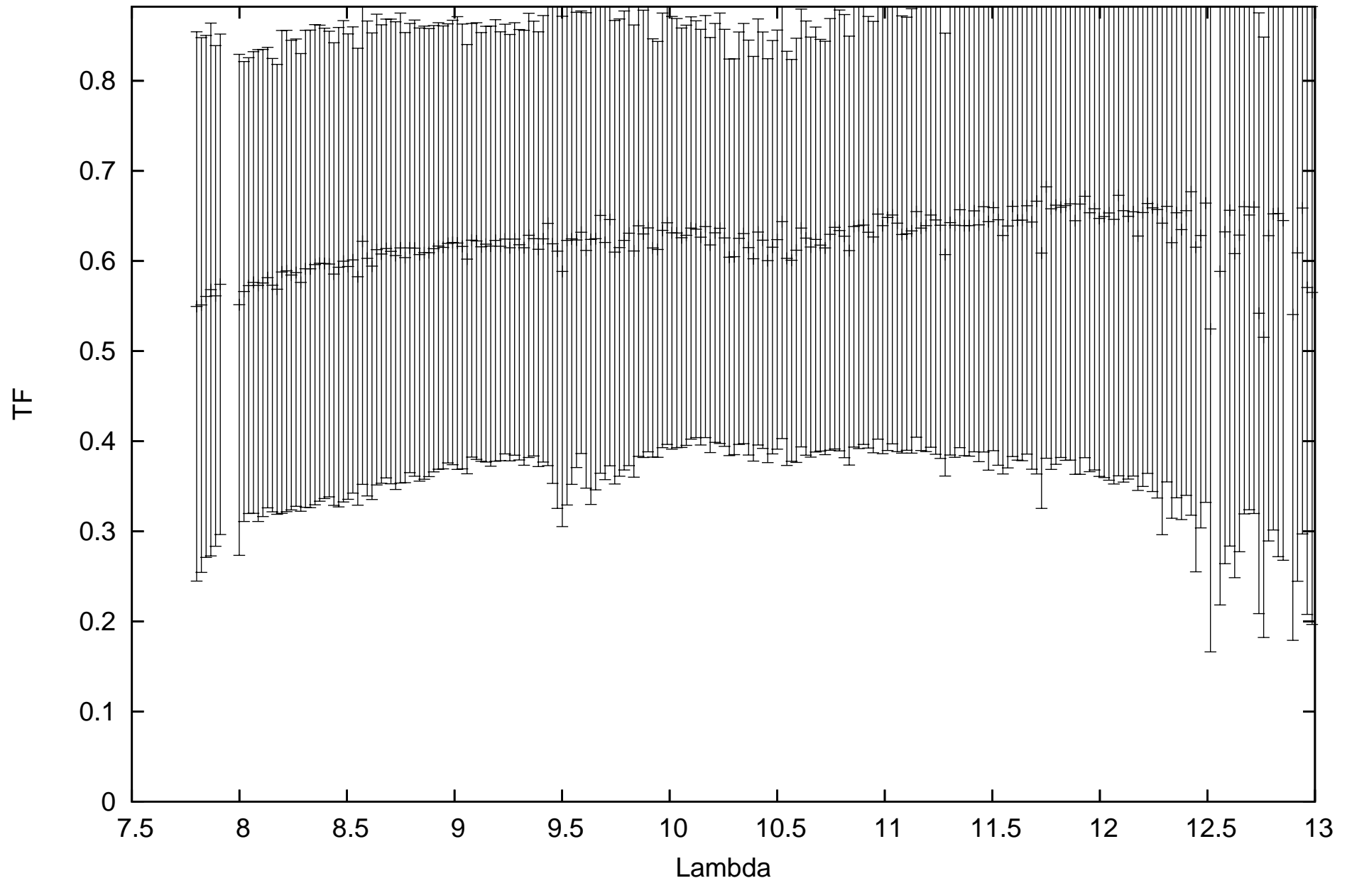
calHD048433_flux1.68_diam2.13_r.MIDI.2011-01-15T03_08_13.000_U2U3
