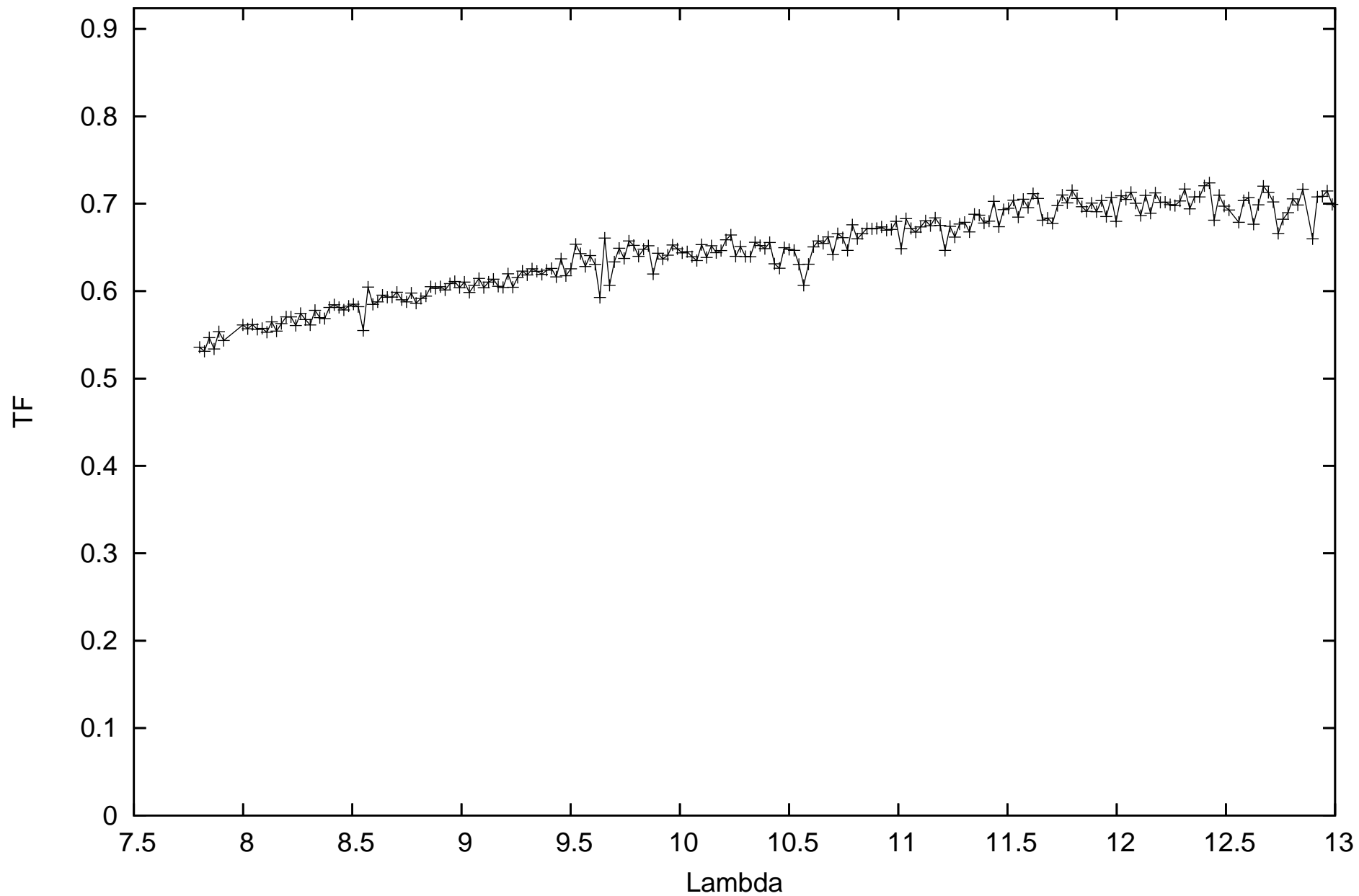
calHDO49161_flux1.49_diam2.44_r.MIDI.2011-01-15T05_55_42.000_U2U3
