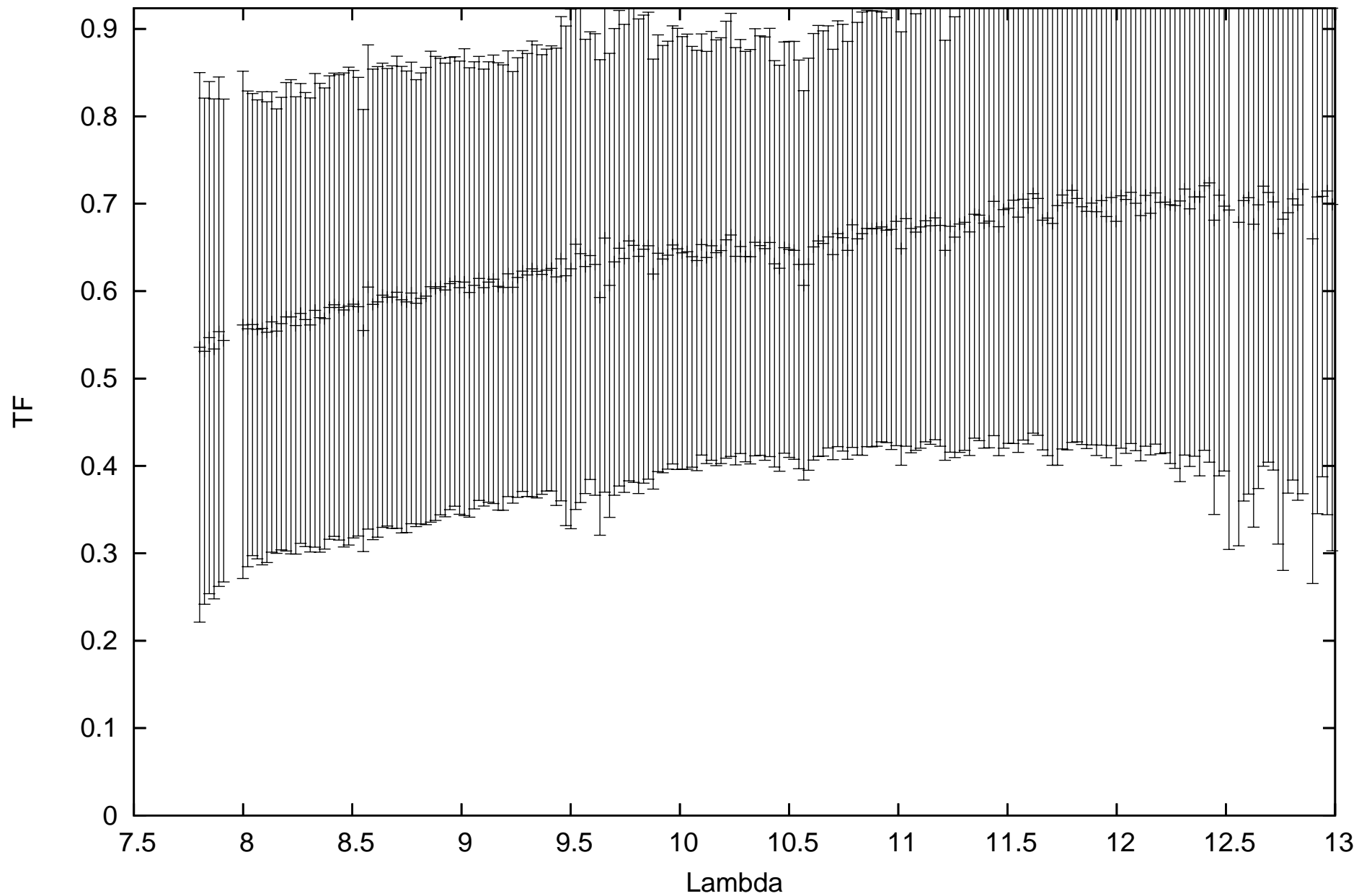
calHD049161_flux1.49_diam2.44_r.MIDI.2011-01-15T05_55_42.000_U2U3
