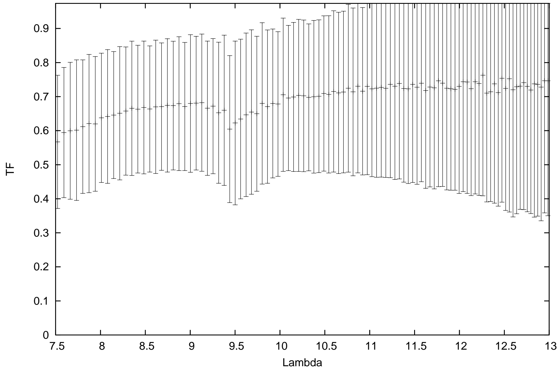
calHD081797_flux-1.49_diam9.14_r.MIDI.2011-01-11T07_22_40.000_D0A1
