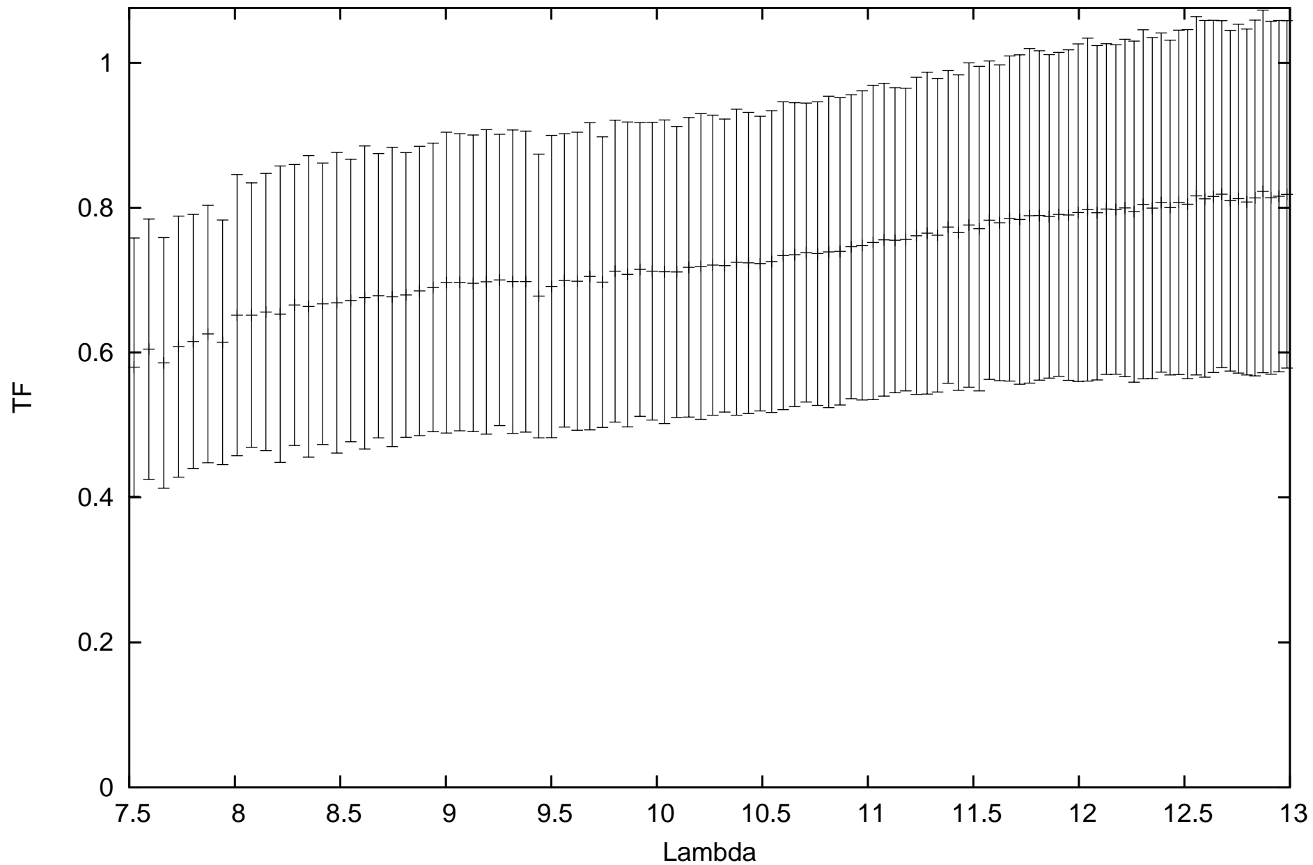
calHD081797_flux-1.49_diam9.14_r.MIDI.2011-01-14T06_01_38.000_U2U3
