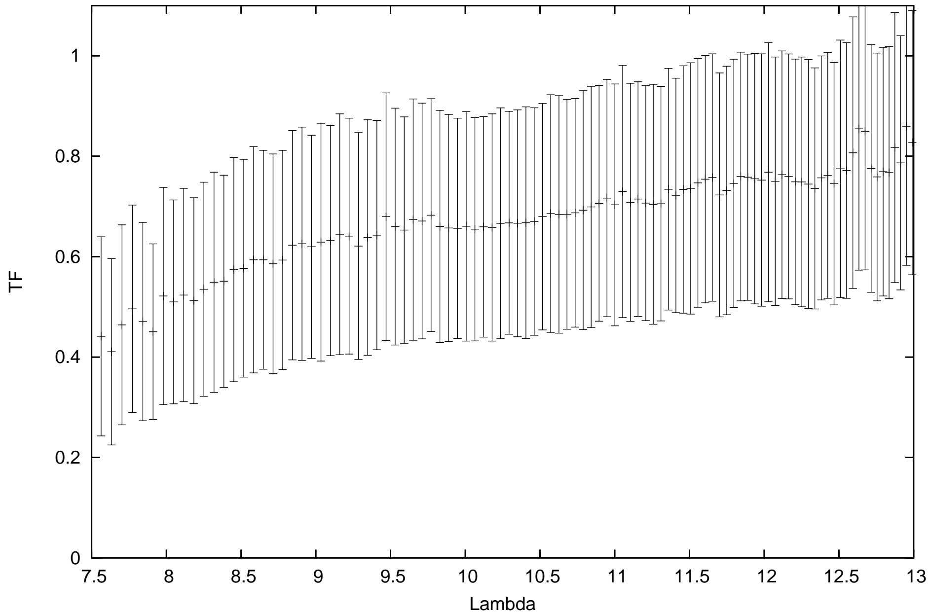
calHD081797_flux-1.49_diam9.14_r.MIDI.2011-01-14T06_10_22.973_U2U3
