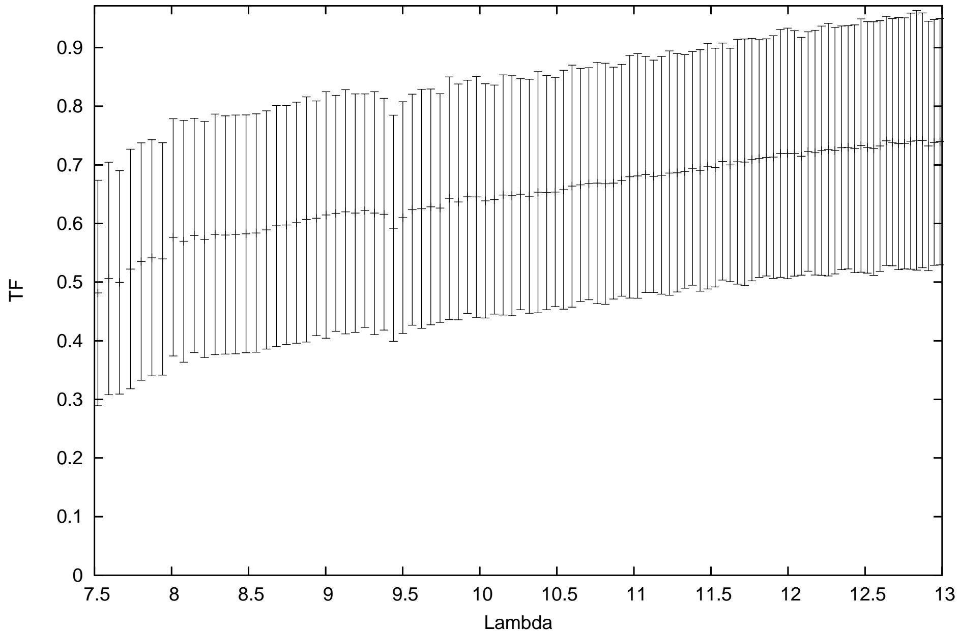
calHD081797_flux-1.49_diam9.14_r.MIDI.2011-01-15T06_25_45.000_U2U3
