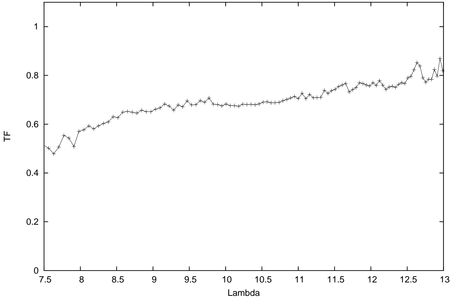
calHD081797_flux-1.49_diam9.14_r.MIDI.2011-01-15T06_34_31.973_U2U3
