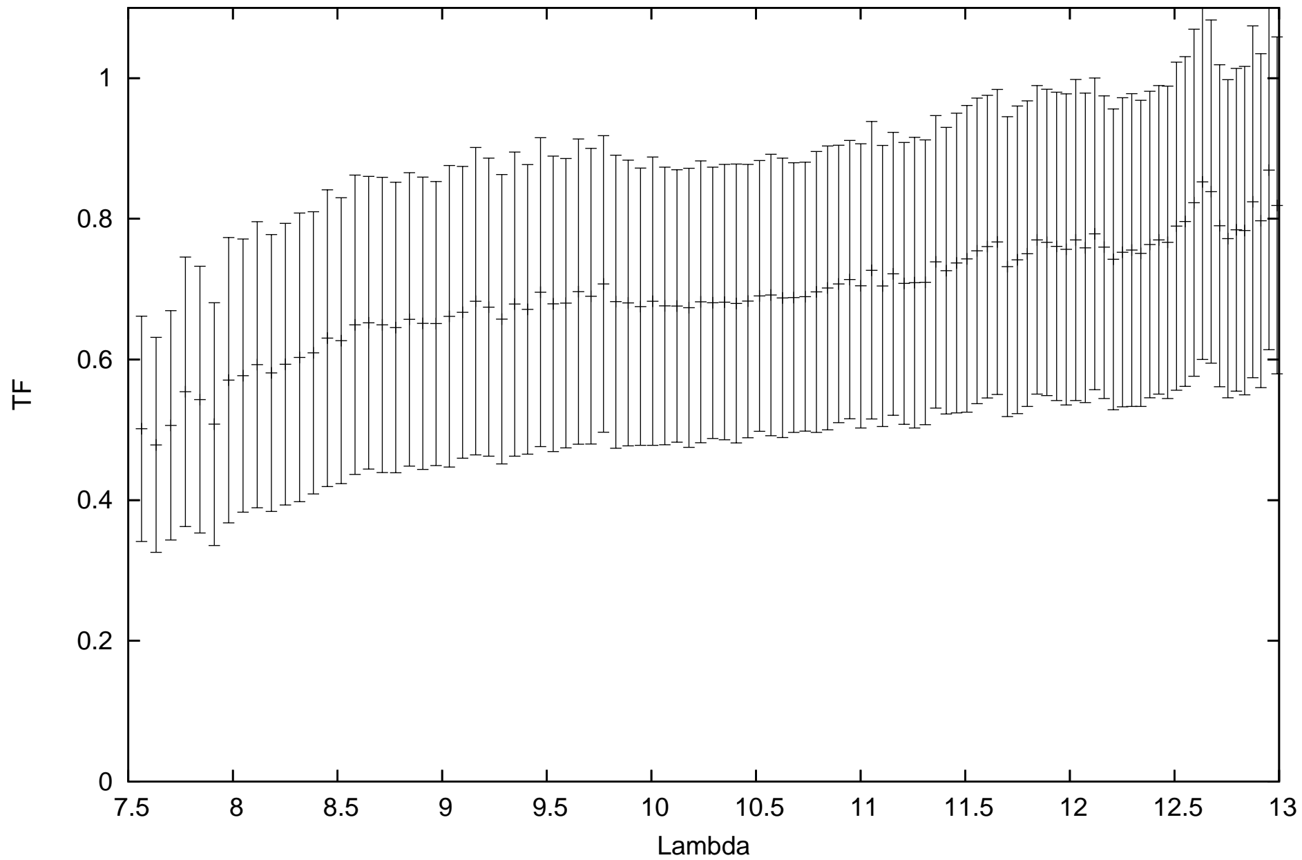
calHD081797_flux-1.49_diam9.14_r.MIDI.2011-01-15T06_34_31.973_U2U3
