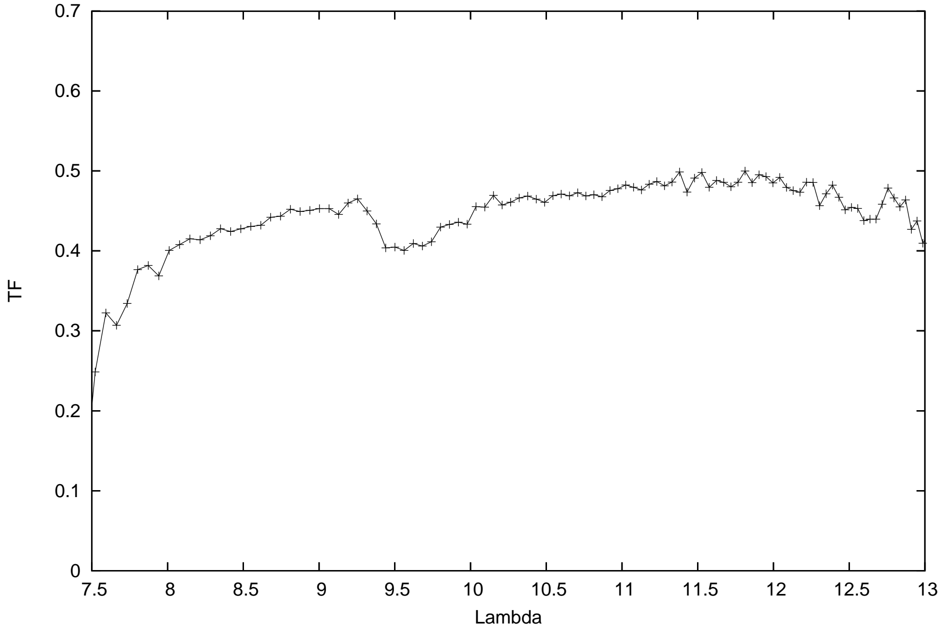
calHD081797_flux-1.49_diam9.14_r.MIDI.2011-02-27T05_36_59.000_D0B2
