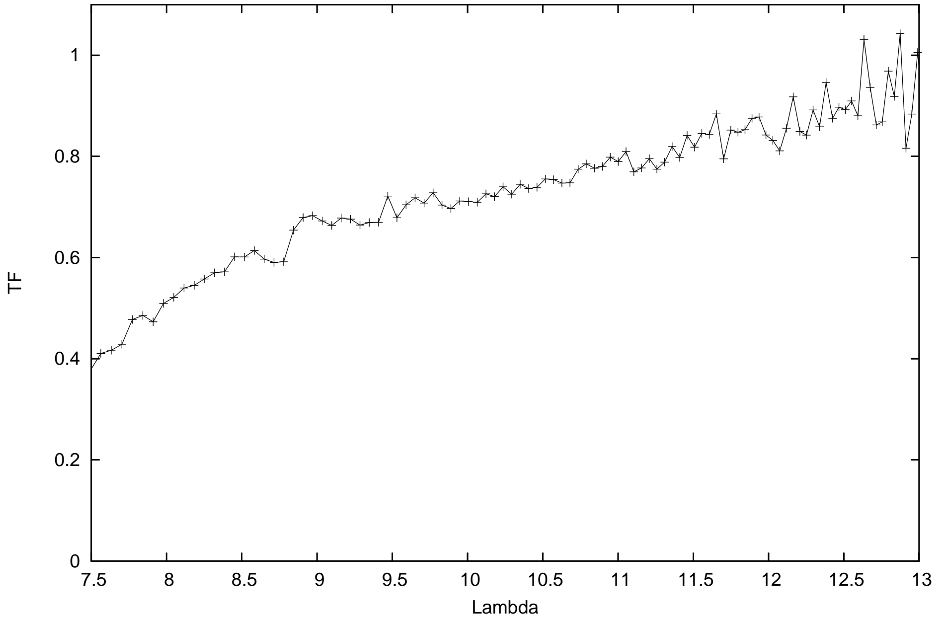
calHD081797_flux-1.49_diam9.14_r.MIDI.2011-03-08T05_02_18.015_H0G0
