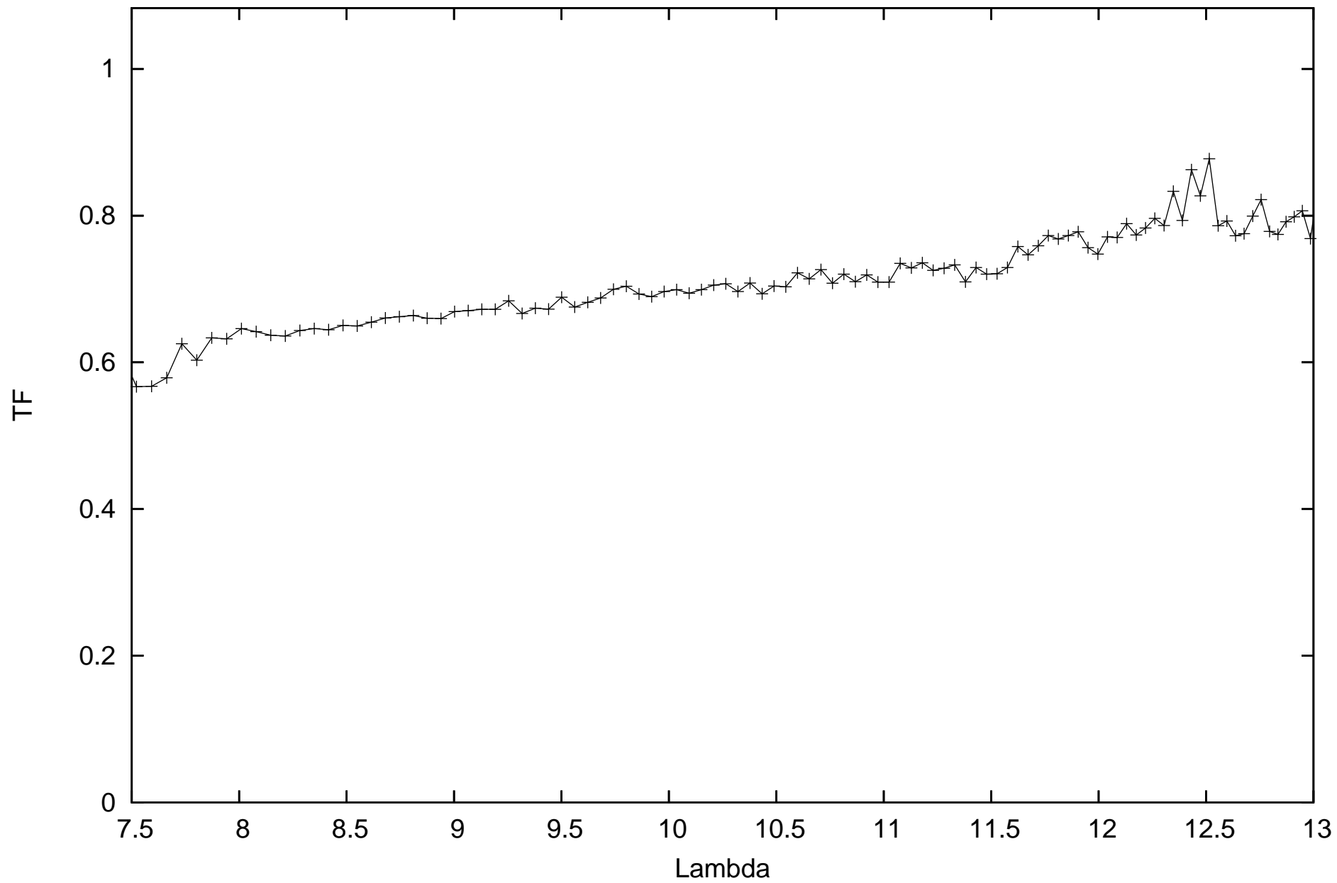
calHD100407_flux1.34_diam2.36_r.MIDI.2011-04-15T04_41_50.000_U2U3
