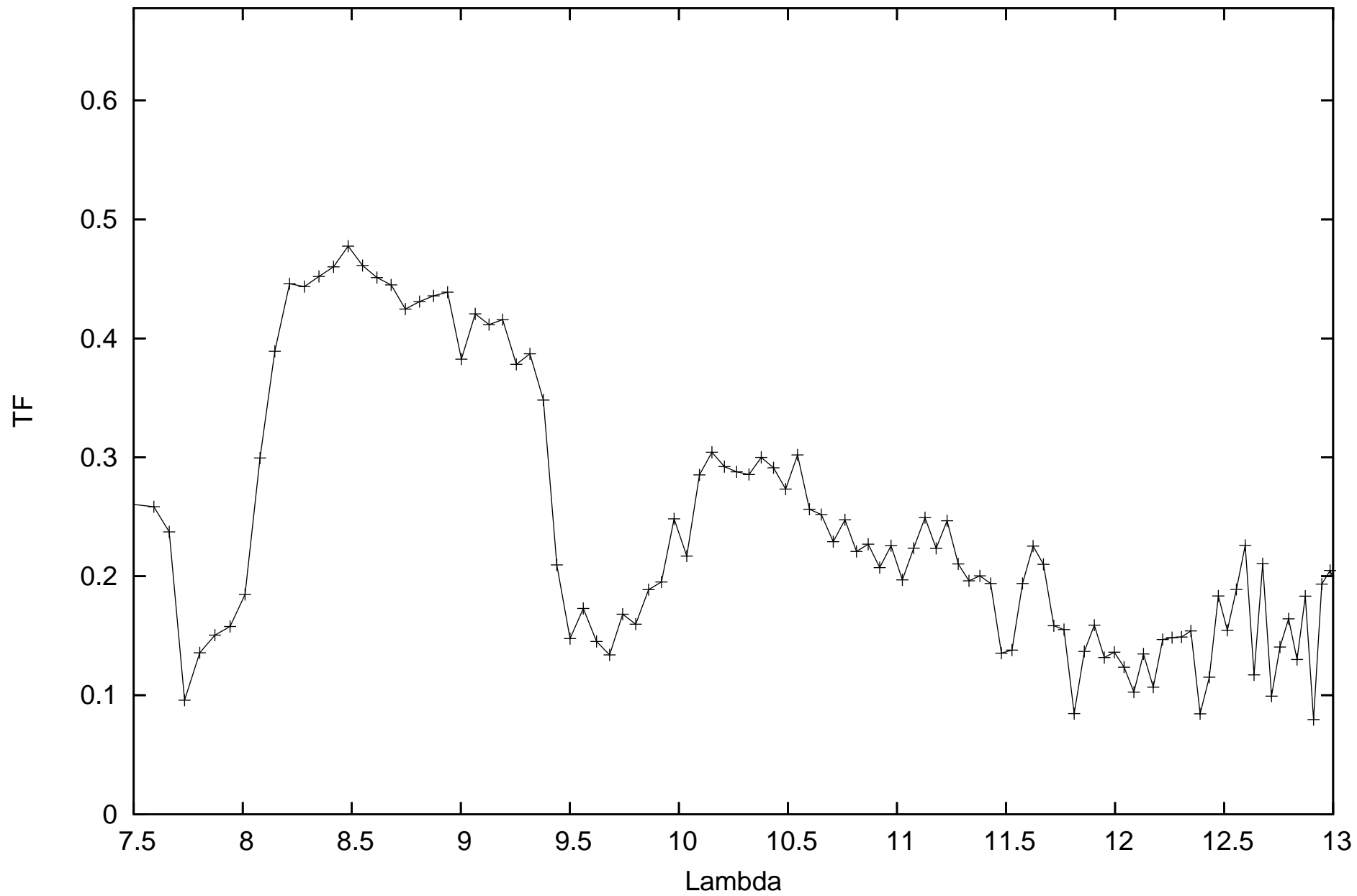
calHD107446_flux0.22_diam4.43_r.MIDI.2011-02-08T07_09_11.000_A011
