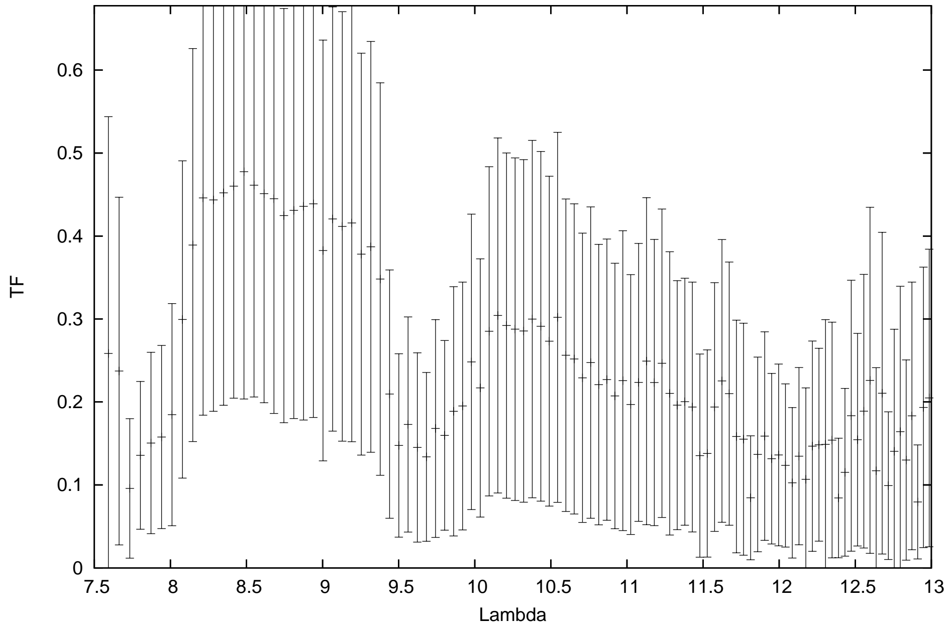
calHD107446_flux0.22_diam4.43_r.MIDI.2011-02-08T07_09_11.000_A011
