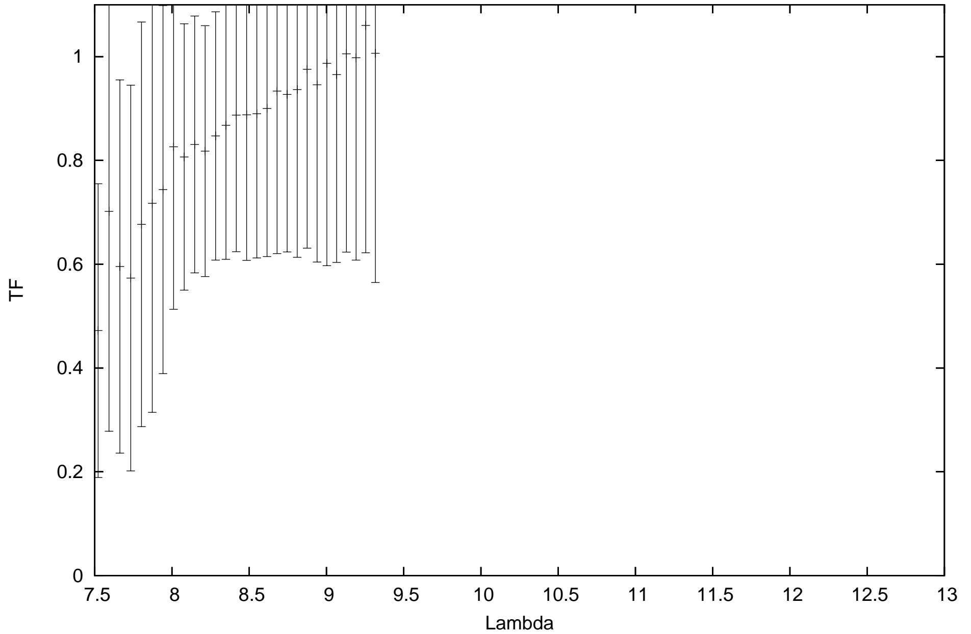
calHD107446_flux0.22_diam4.43_r.MIDI.2011-03-06T07_00_40.000_H0G0
