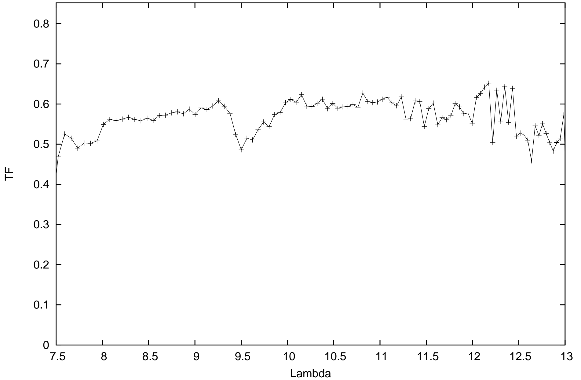
calHD107446_flux0.22_diam4.43_r.MIDI.2011-04-23T04_23_27.000_K011
