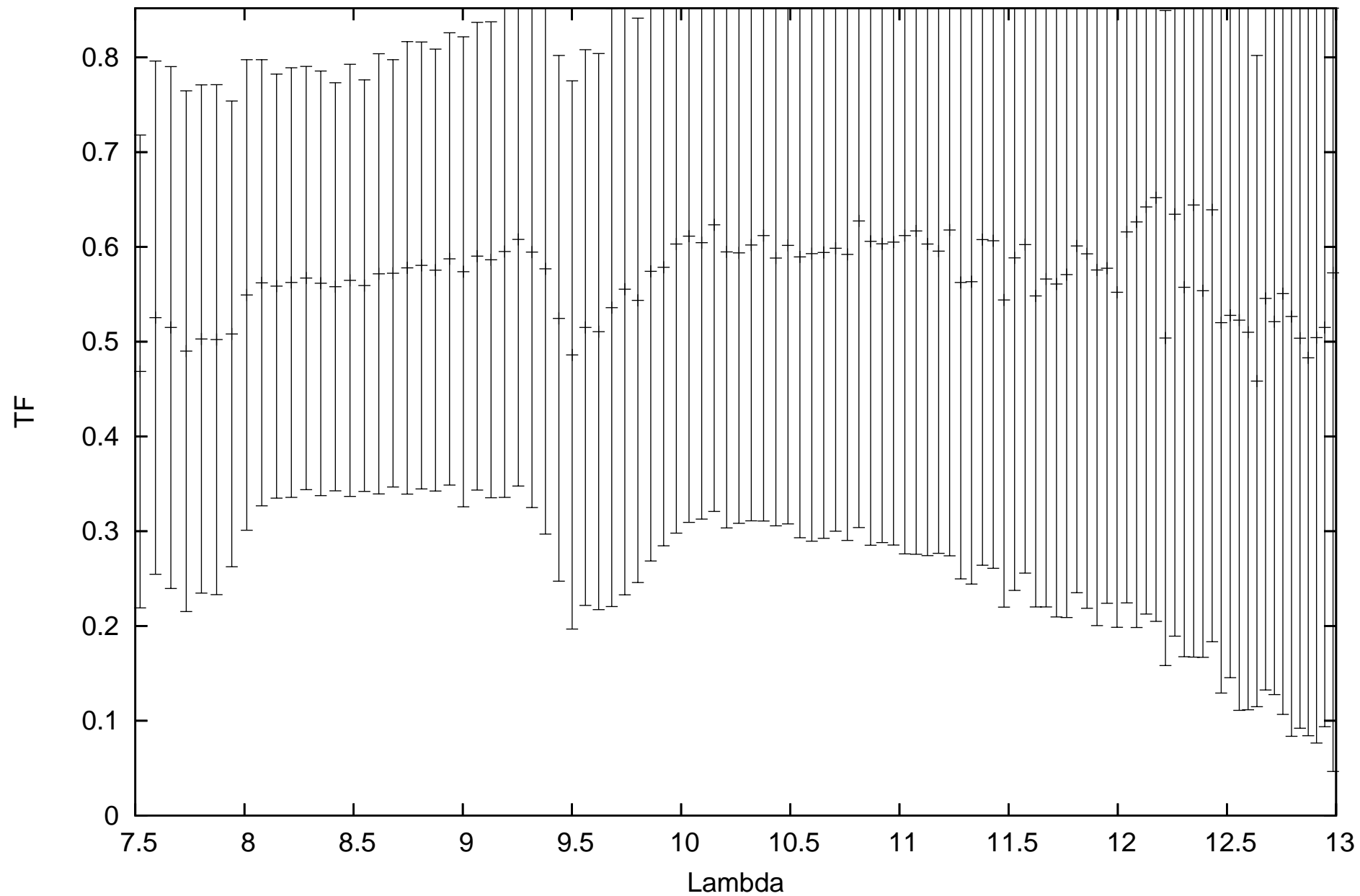
calHD107446_flux0.22_diam4.43_r.MIDI.2011-04-23T04_23_27.000_K0I1
