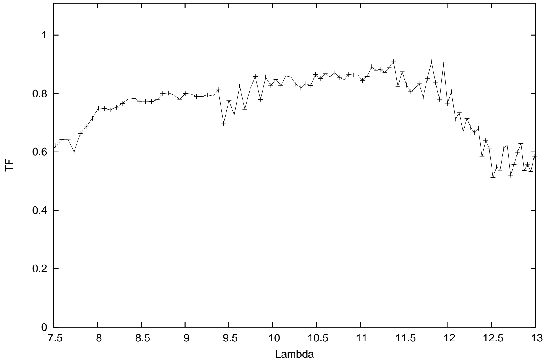
calHD107446_flux0.22_diam4.43_r.MIDI.2011-05-03T05_24_44.000_G111
