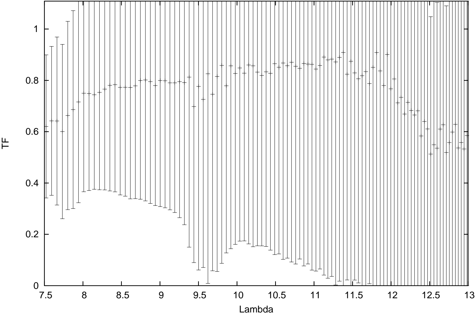
calHD107446_flux0.22_diam4.43_r.MIDI.2011-05-03T05_24_44.000_G111
