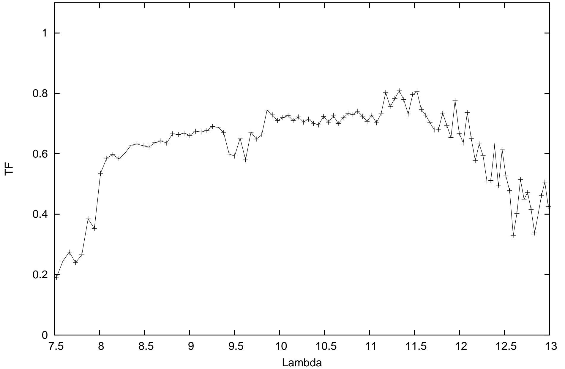
calHD107446_flux0.22_diam4.43_r.MIDI.2011-05-09T05_40_05.000_D0B2
