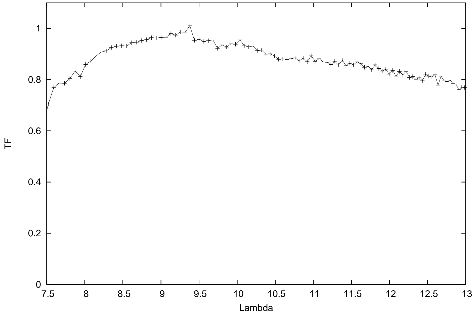
calHD107446_flux0.22_diam4.43_r.MIDI.2011-12-12T08_21_44.000_U1U4
