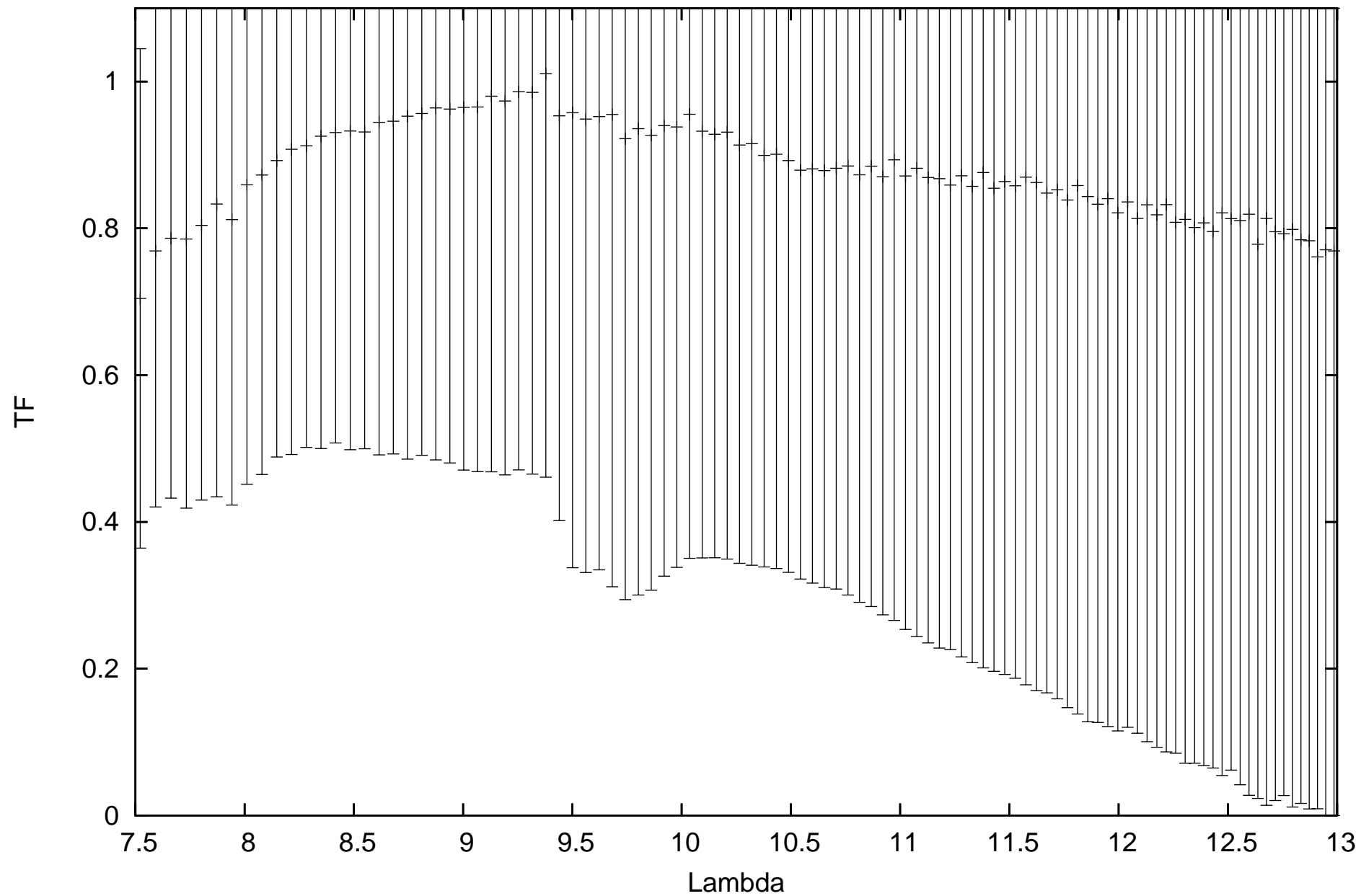
calHD107446_flux0.22_diam4.43_r.MIDI.2011-12-12T08_21_44.000_U1U4
