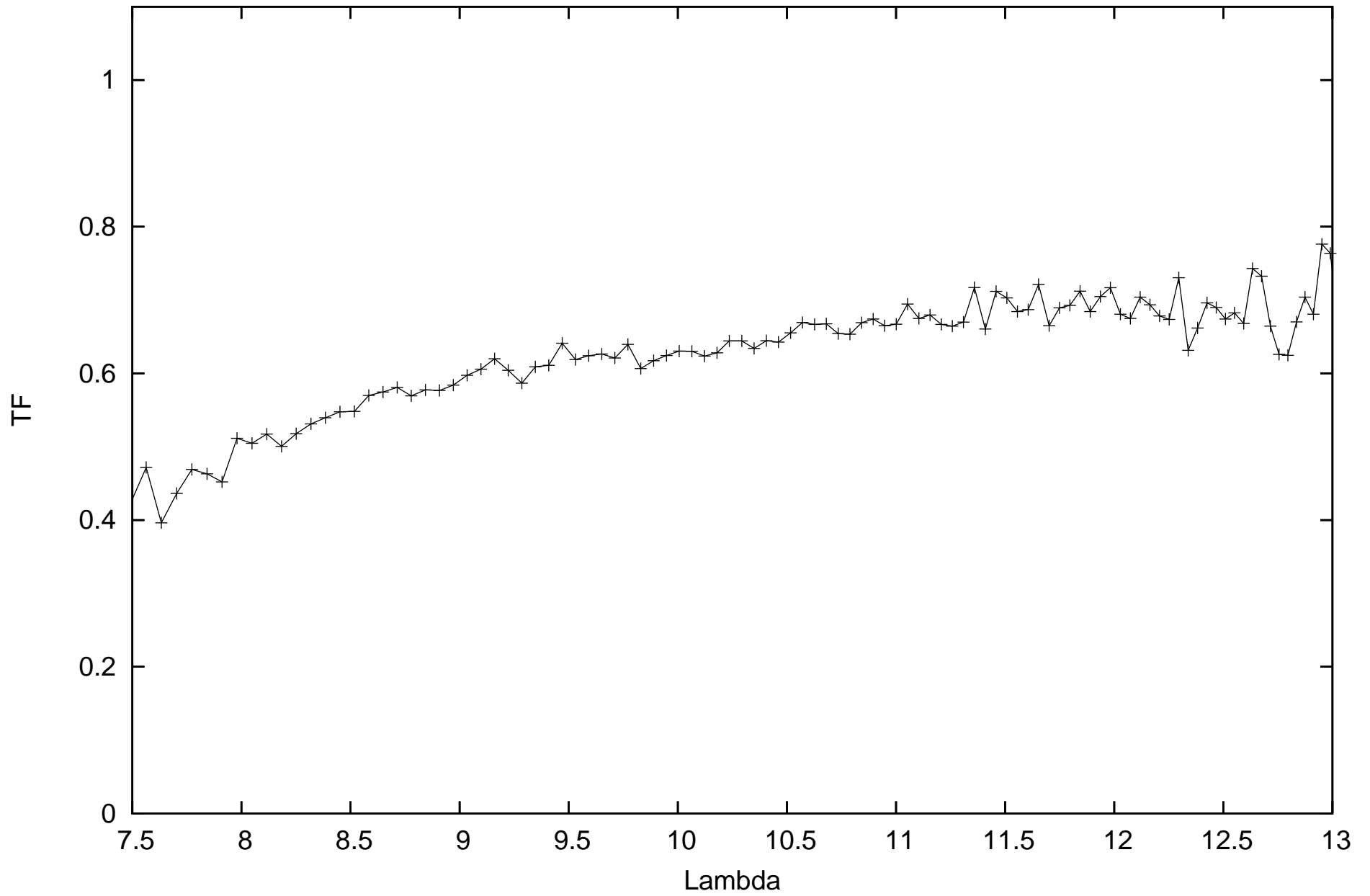
calHD120323_flux-2.02_diam13.25_r.MIDI.2011-05-09T06_11_42.015_C1A1
