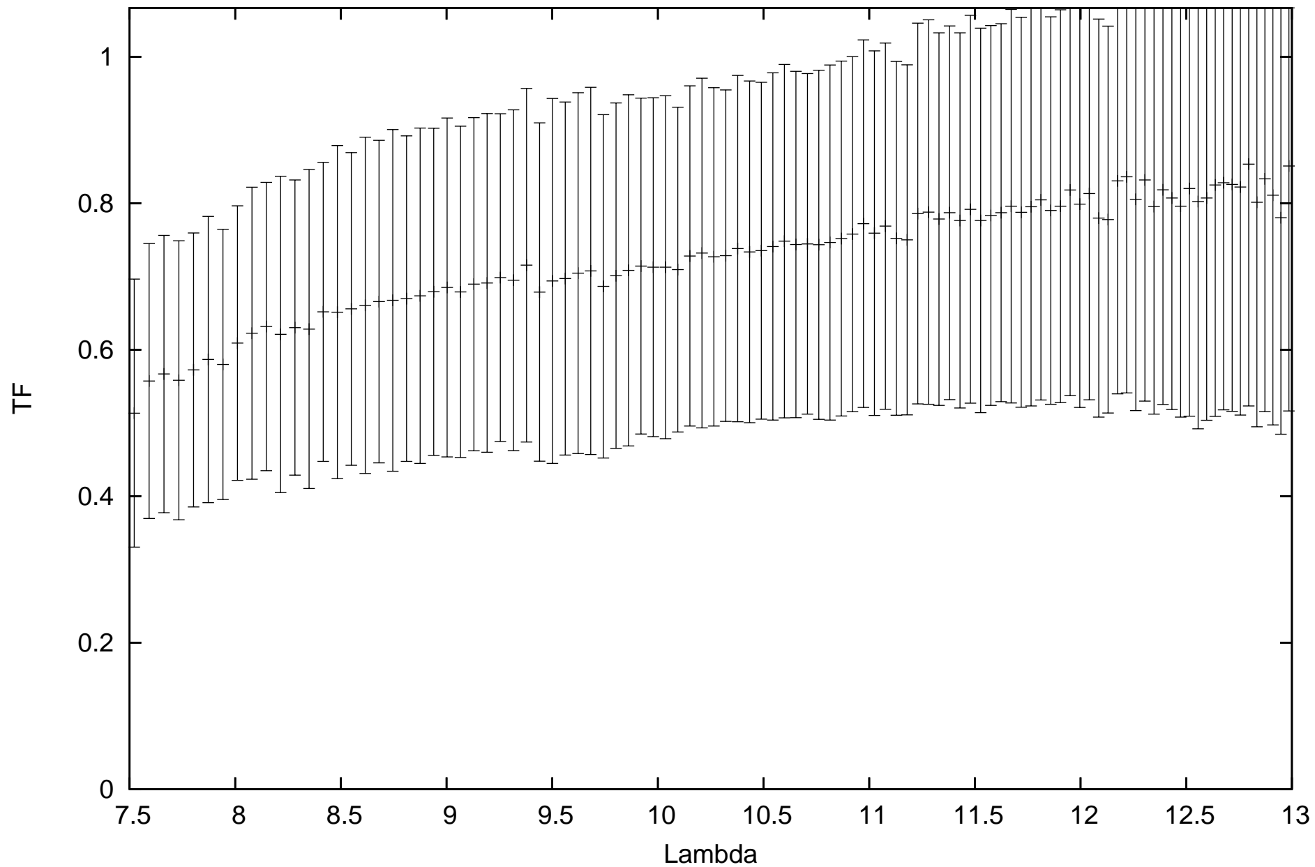
calHD120404_flux1.19_diam2.96_r.MIDI.2011-03-20T03_08_08.000_U2U3
