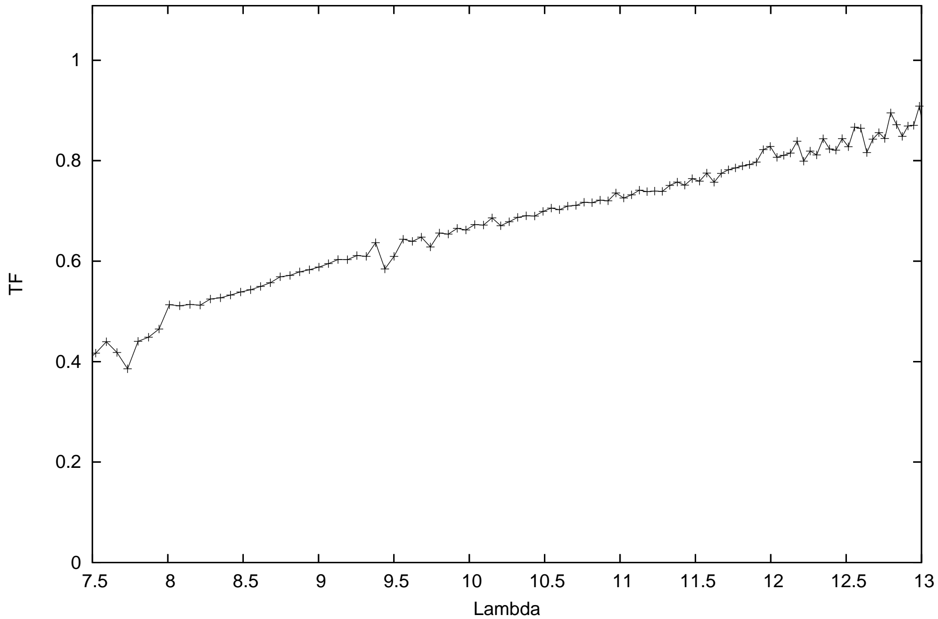
calHD120404_flux1.19_diam2.96_r.MIDI.2011-04-17T00_04_07.000_U3U4
