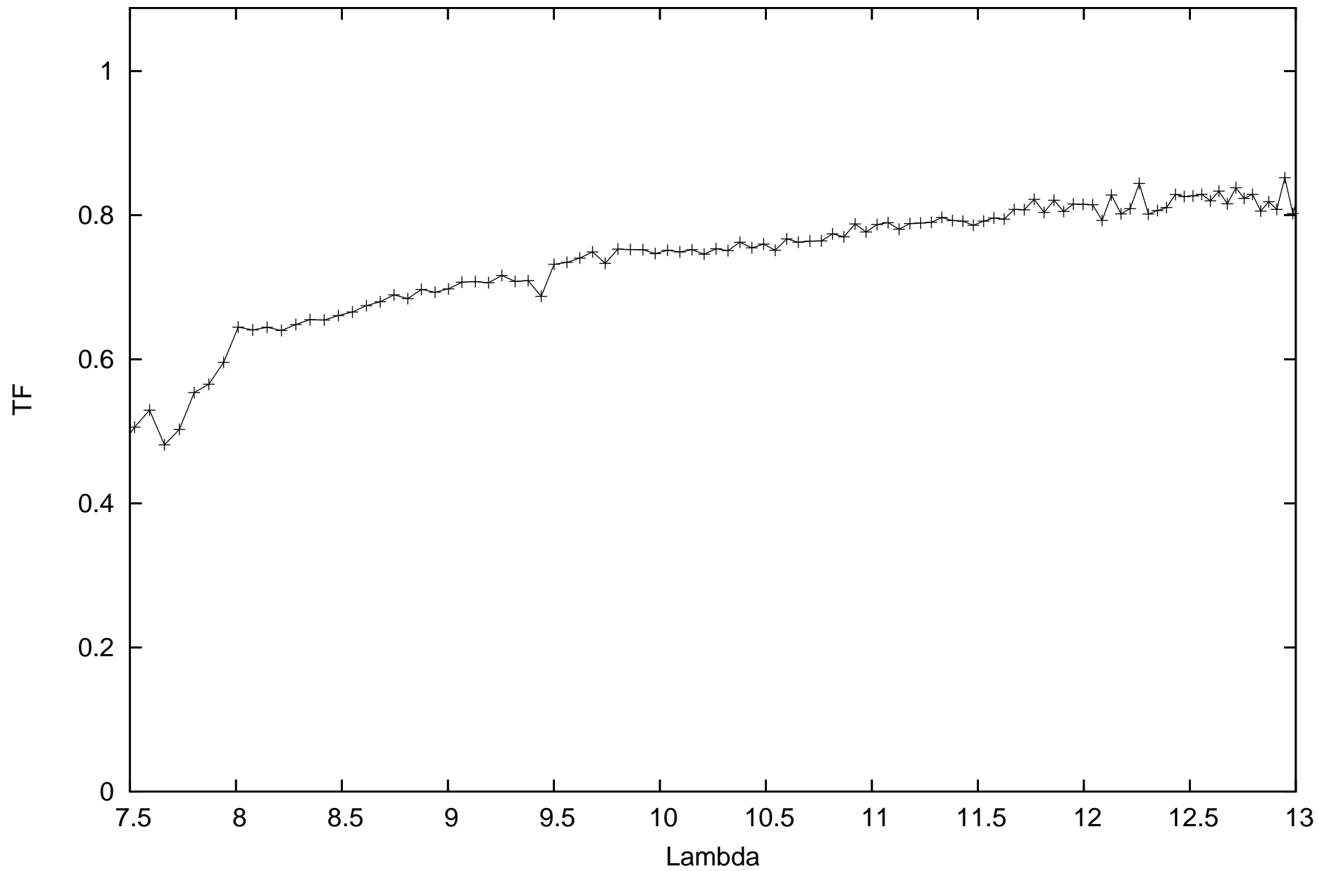
calHD120404_flux1.19_diam2.96_r.MIDI.2011-04-18T09_12_58.000_U2U4
