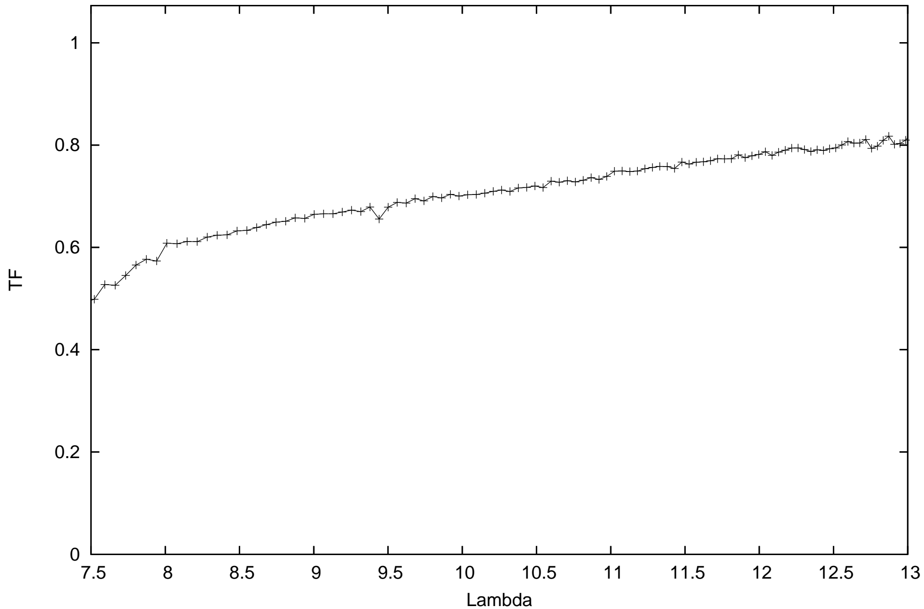
calHD123139_flux-0.39_diam5.34_r.MIDI.2011-03-18T07_48_17.000_U1U2
