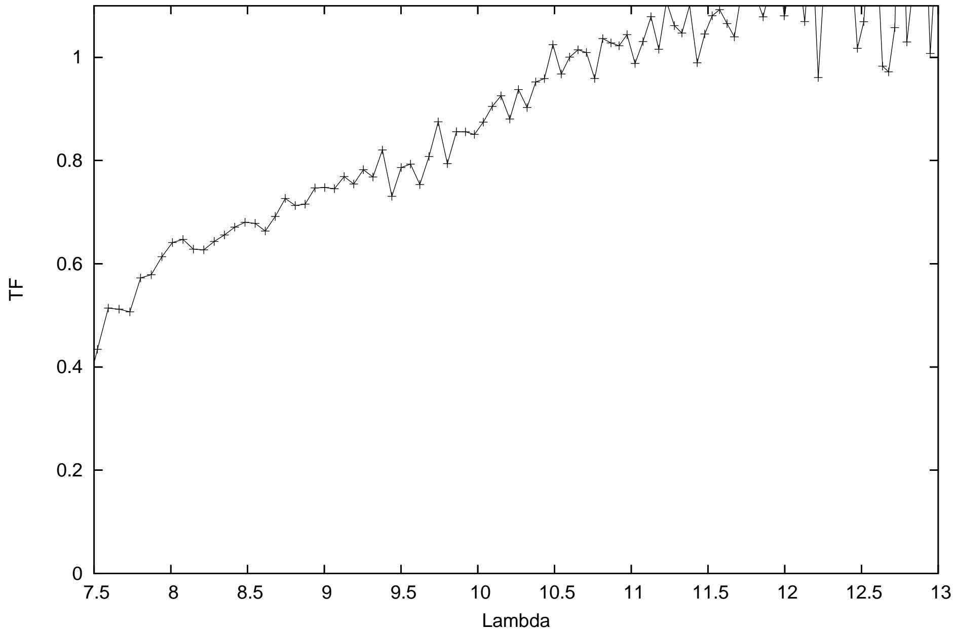
calHD123139_flux-0.39_diam5.34_r.MIDI.2011-04-08T02_08_17.000_K0I1
